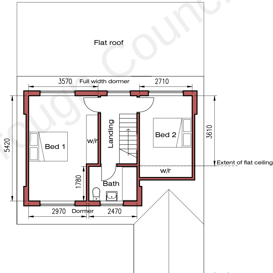
First Floor
