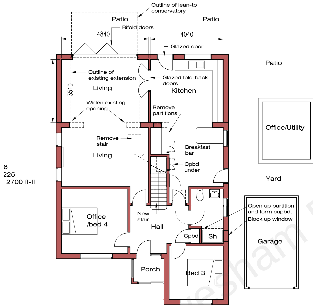
Ground Floor
