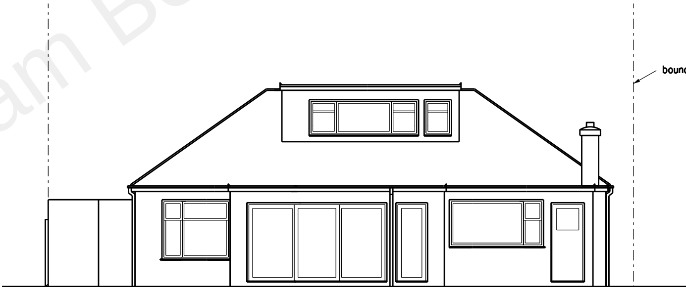
REAR ELEVATION
