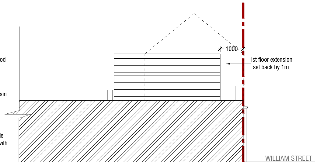
PROPOSED ELEVATION (E2)
