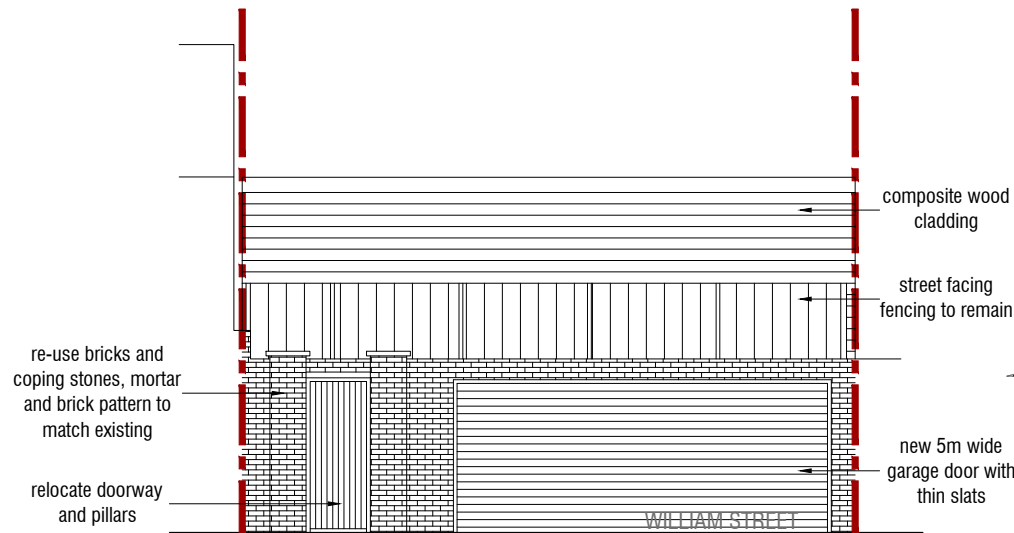
PROPOSED ELEVATION (E1)
