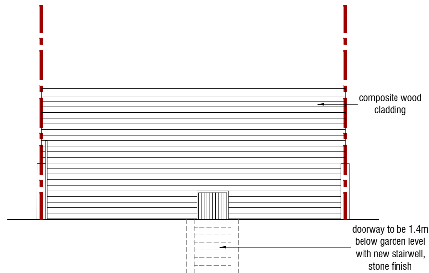
PROPOSED ELEVATION (E3)
