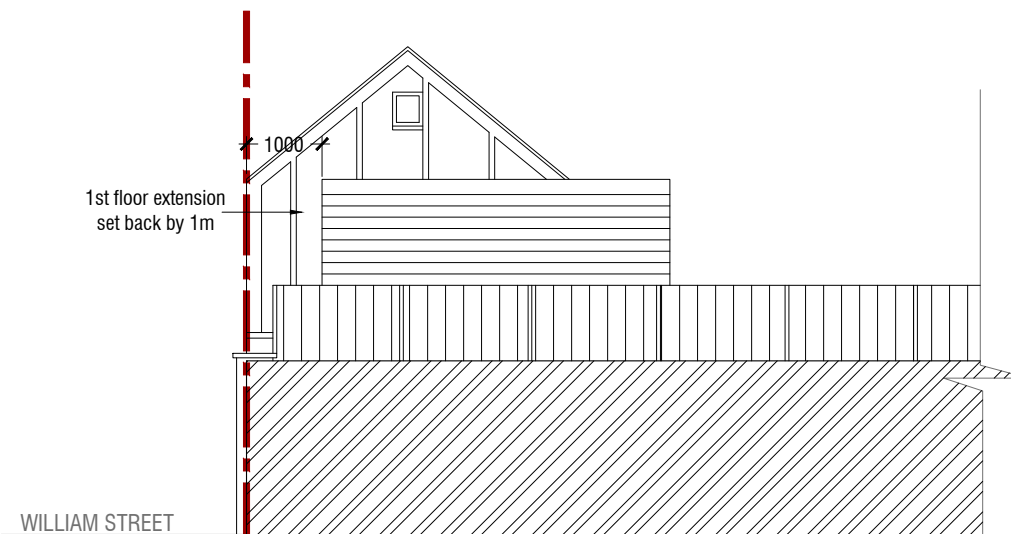
PROPOSED ELEVATION (E4)
