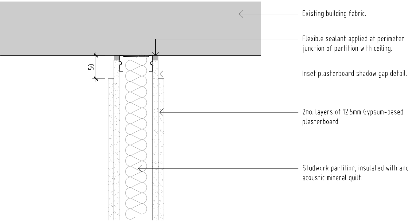
Shadow Gap Junction Detail Non-loadbearing internal partition scale 1:5
