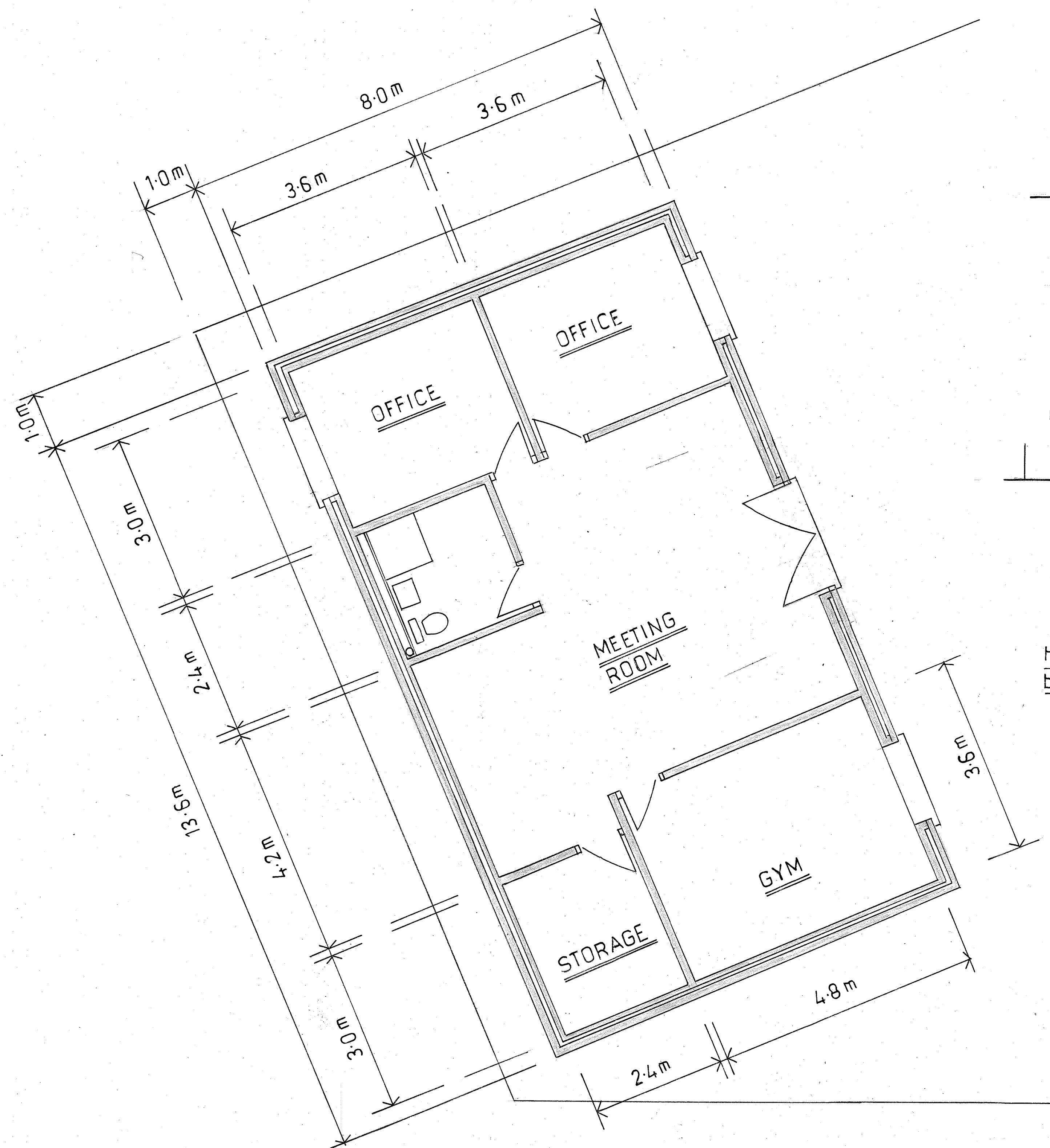
FLOOR PLAN
