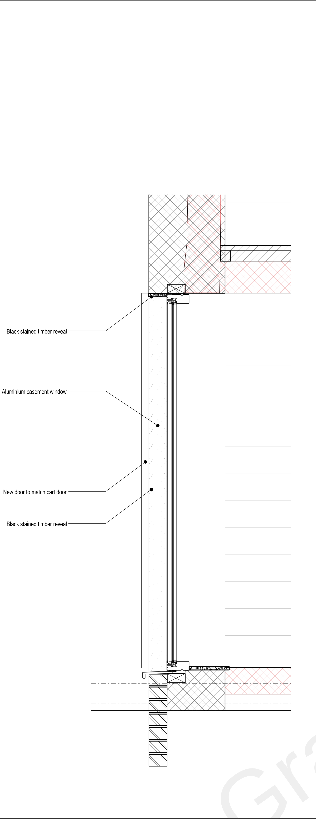
01 SECTION DETAIL
