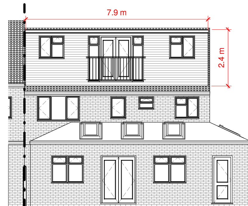
3 Proposed Rear Elevation. 1 : 100
