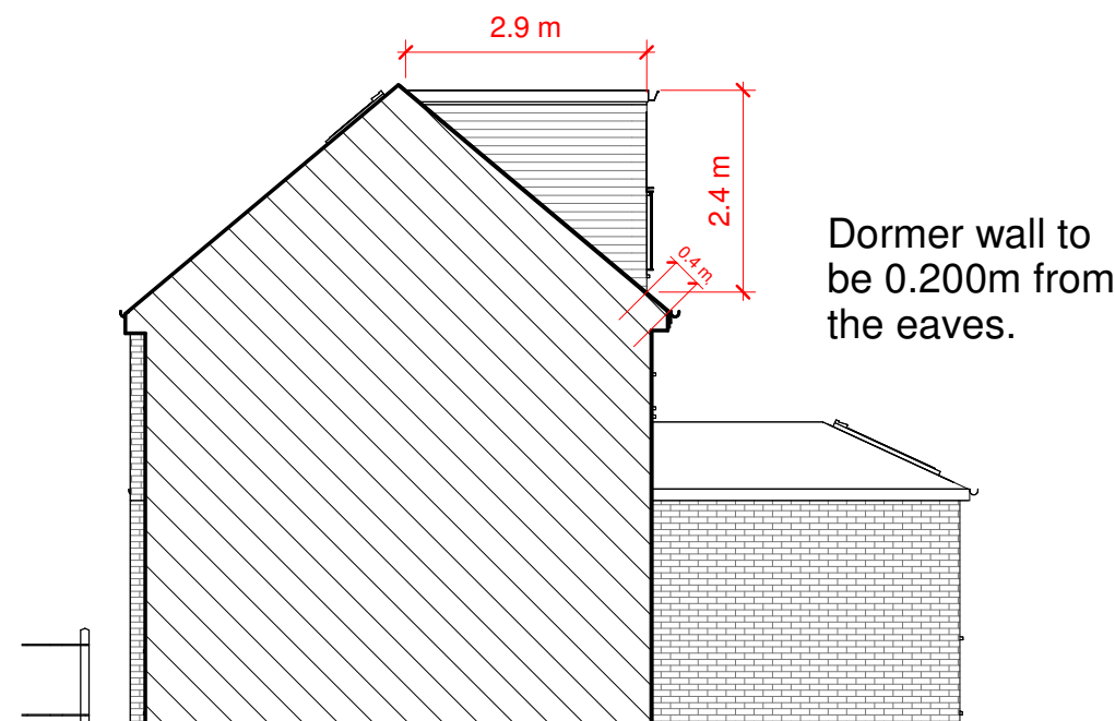
2 Proposed Side Elevation II 1 : 100
