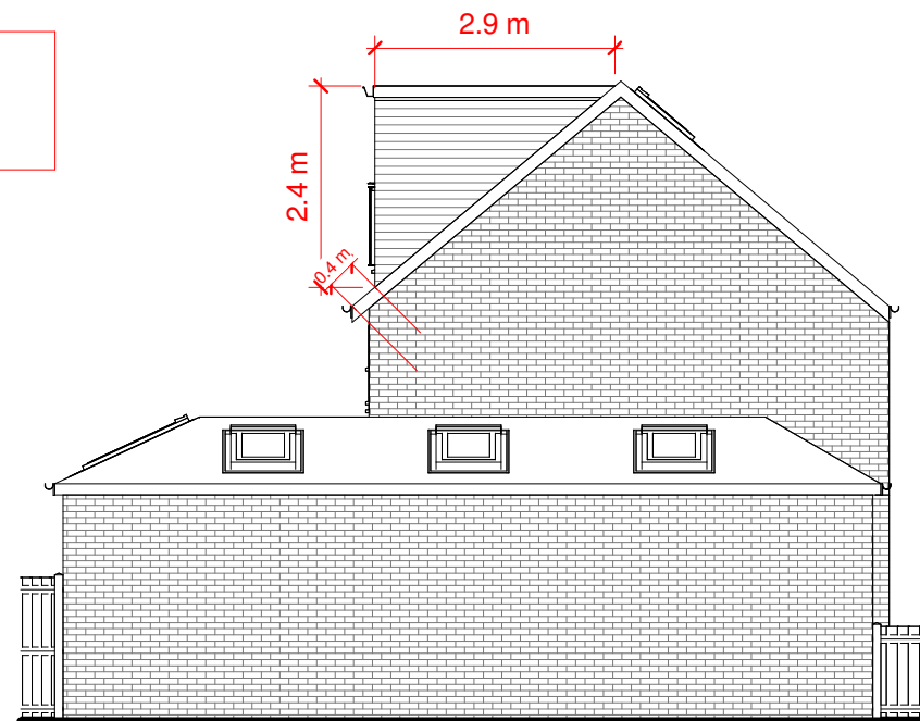
4 Proposed Side Elevation. 1 : 100
