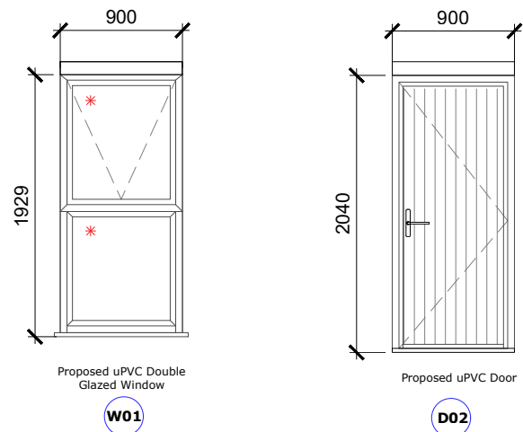
2 Proposed Door and Window Schedule
