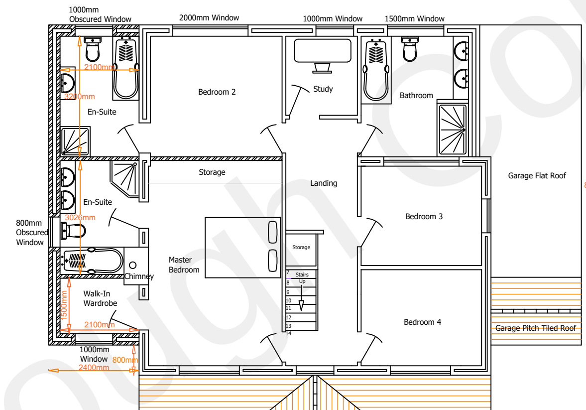
Proposed First Floor Plan 1:100
