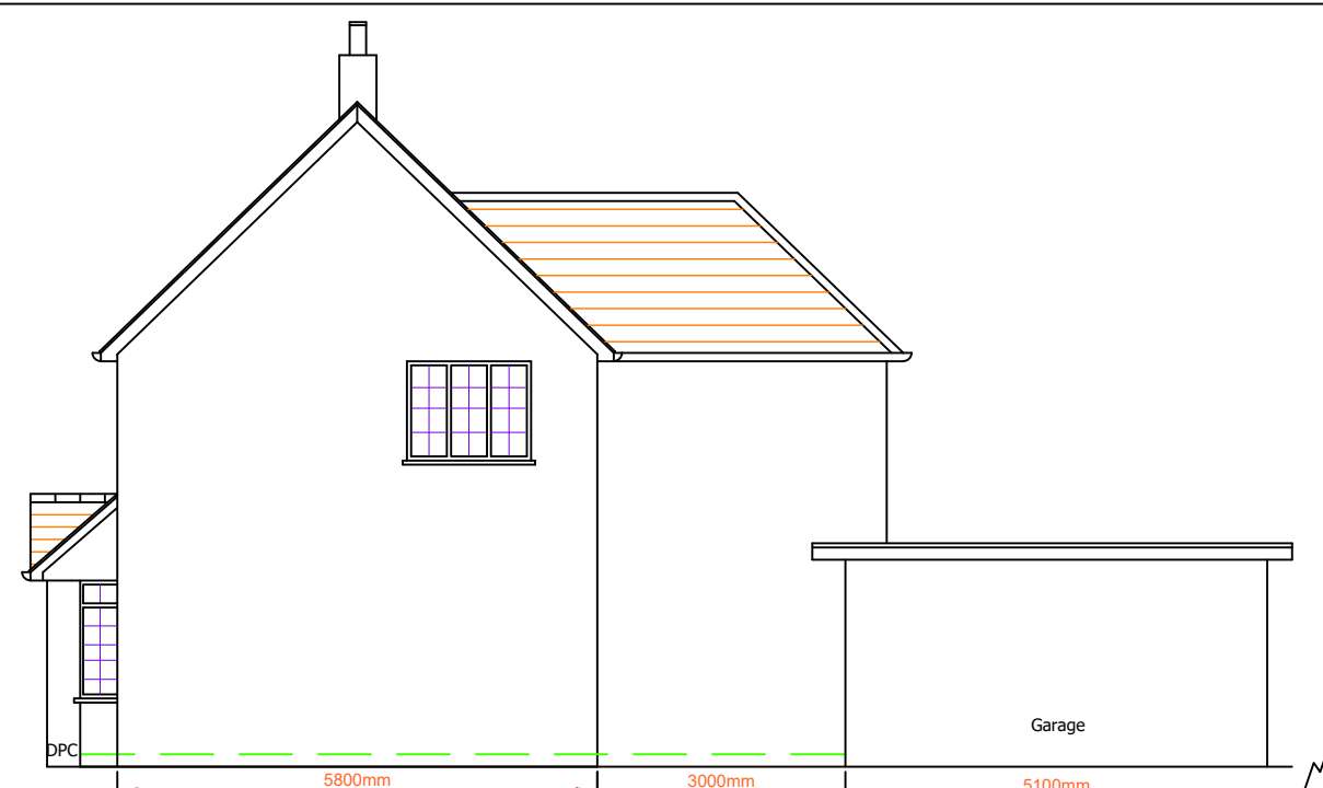
Existing Side (North) Elevation 1:100
