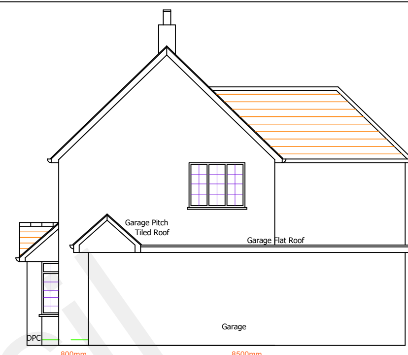
Proposed Side (North) Elevation 1:100
