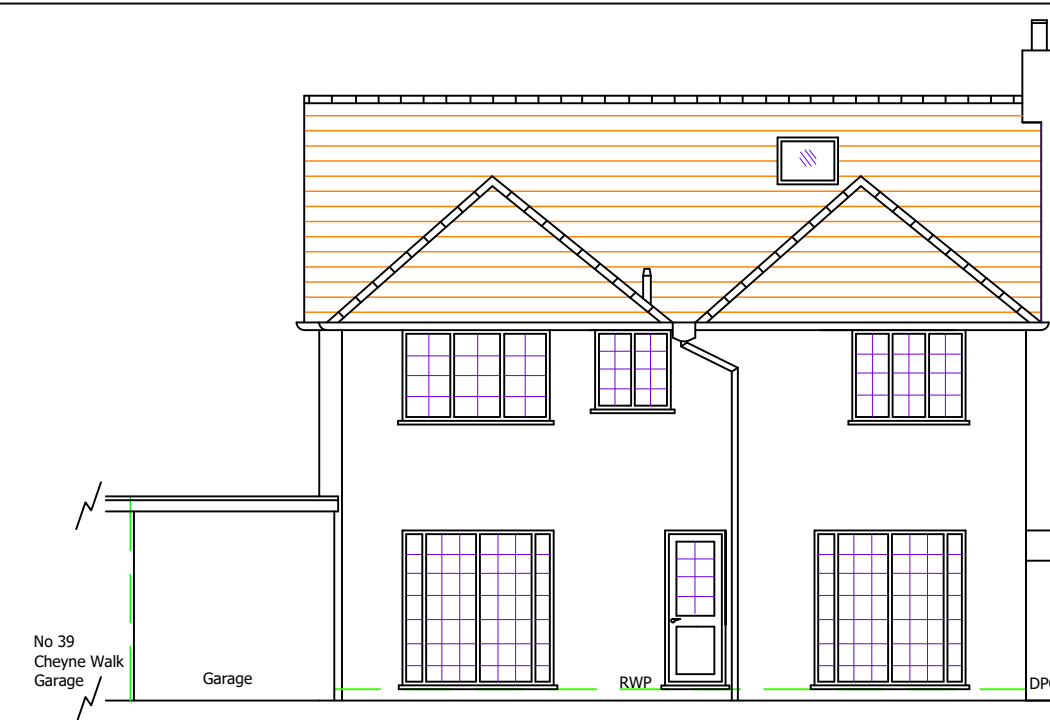
Existing Rear (West) Elevation 1:100
