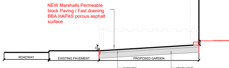
PROPOSED SECTION
