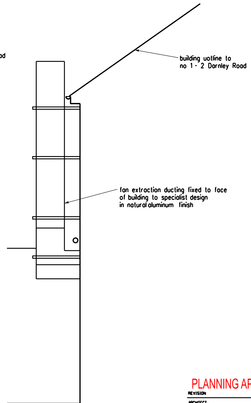
SIDE ELEVATION TO YARD
