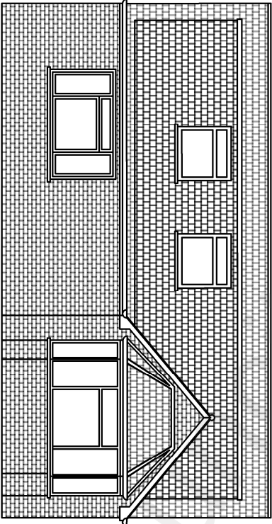
Proposed Front Elevation Scale 1/100
