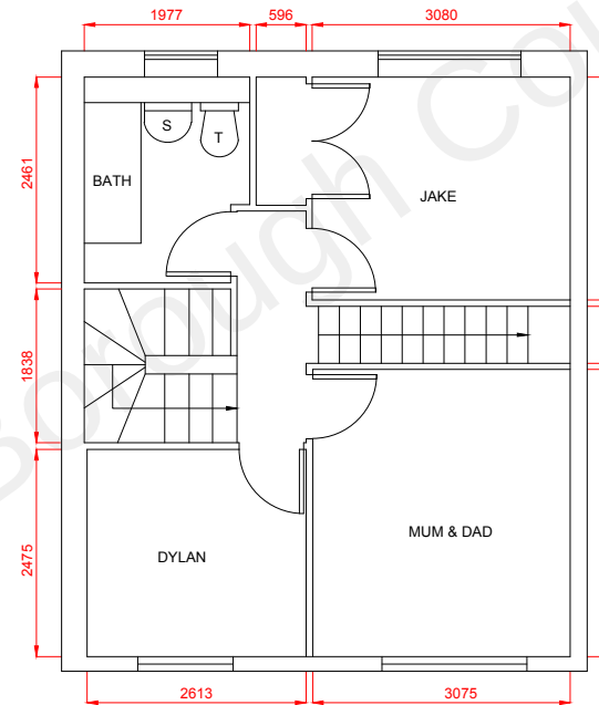
PROPOSED FIRST FLOOR
