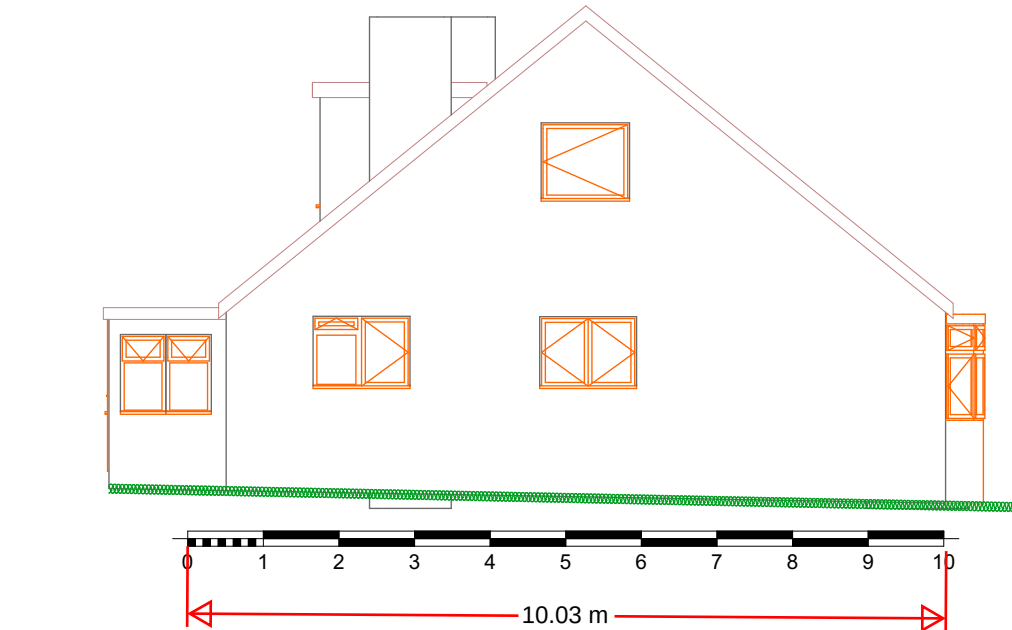
4 South Elevation Existing 1:100
