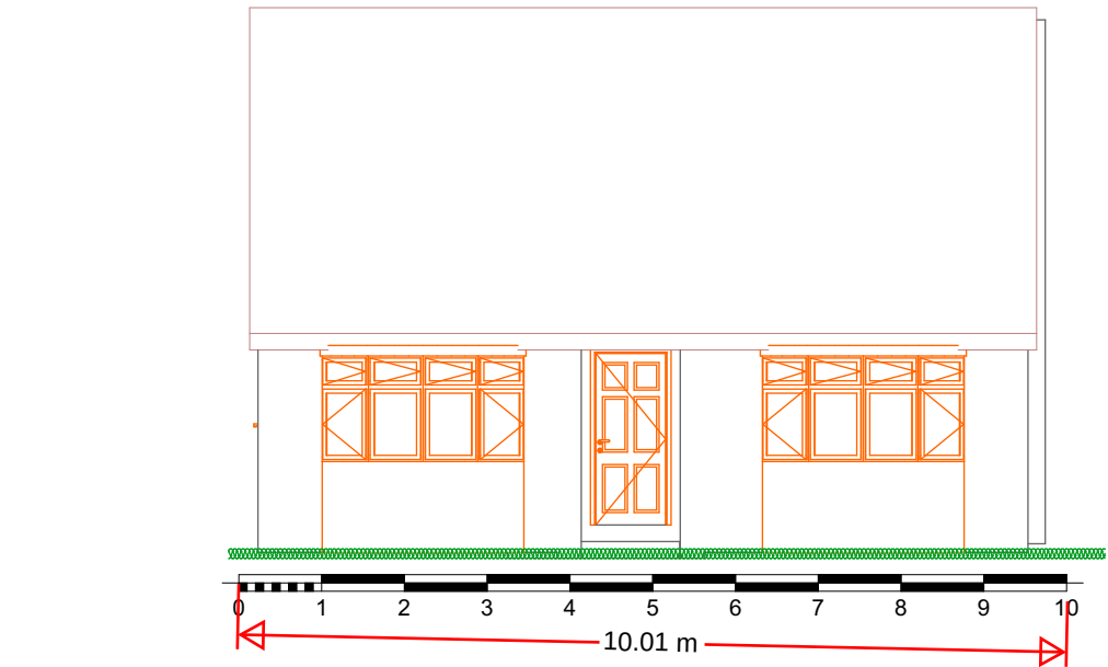
1 East Elevation Existing 1:100
