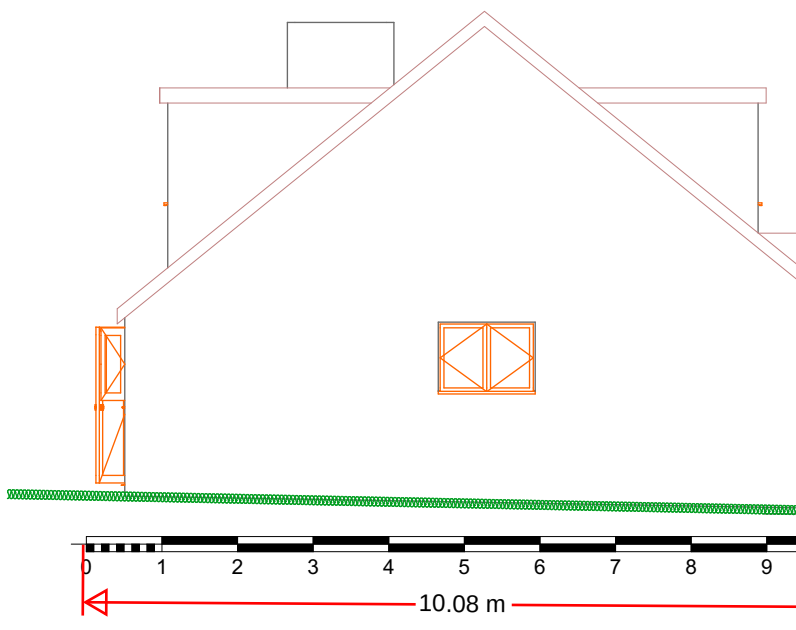
9 South Elevation Proposed 1:100
