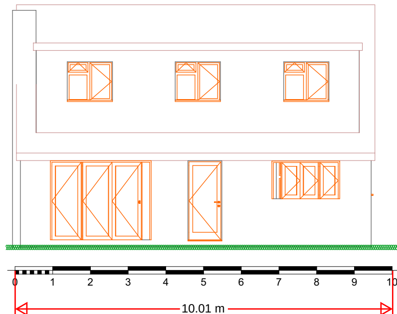
7 West Elevation Proposed 1:100
