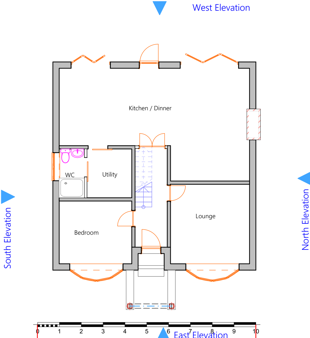
10 GF Ground Floor Proposed 1:100
