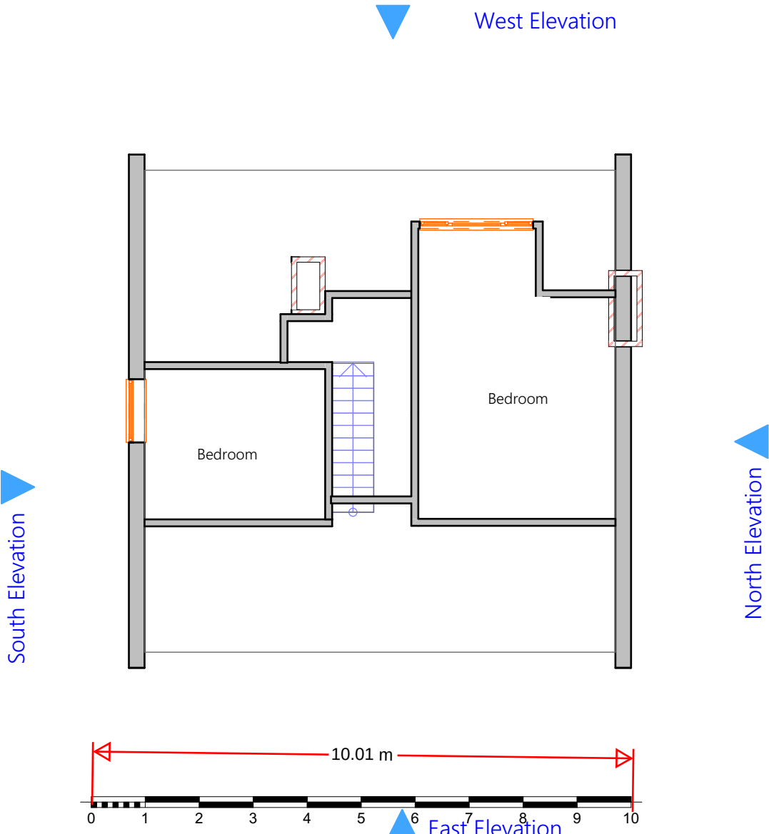
11 01 First Floor Existing 1:100
