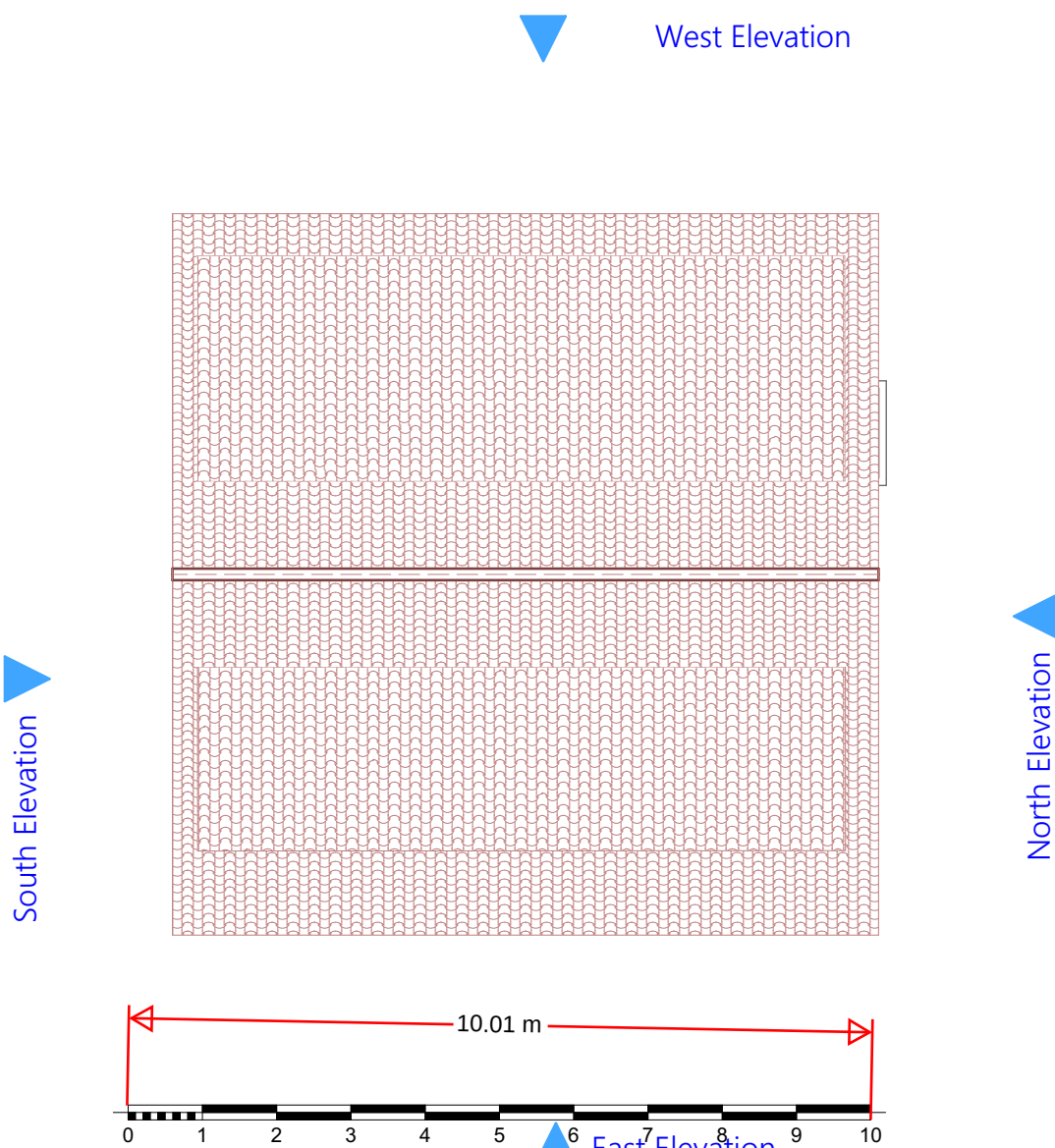
14 Roof Proposed 1:100
