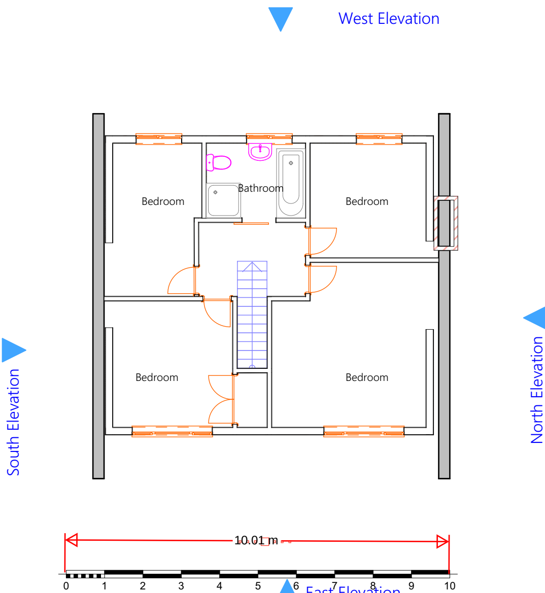
12 01 First Floor Proposed 1:100
