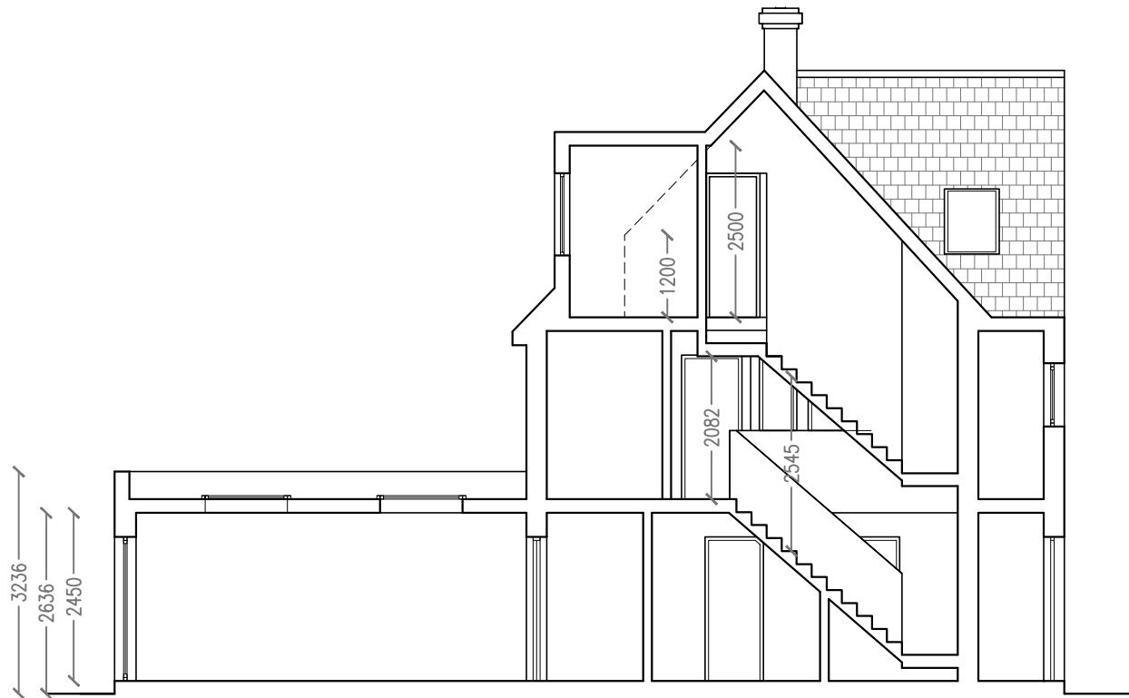
Existing Long Section AA'
