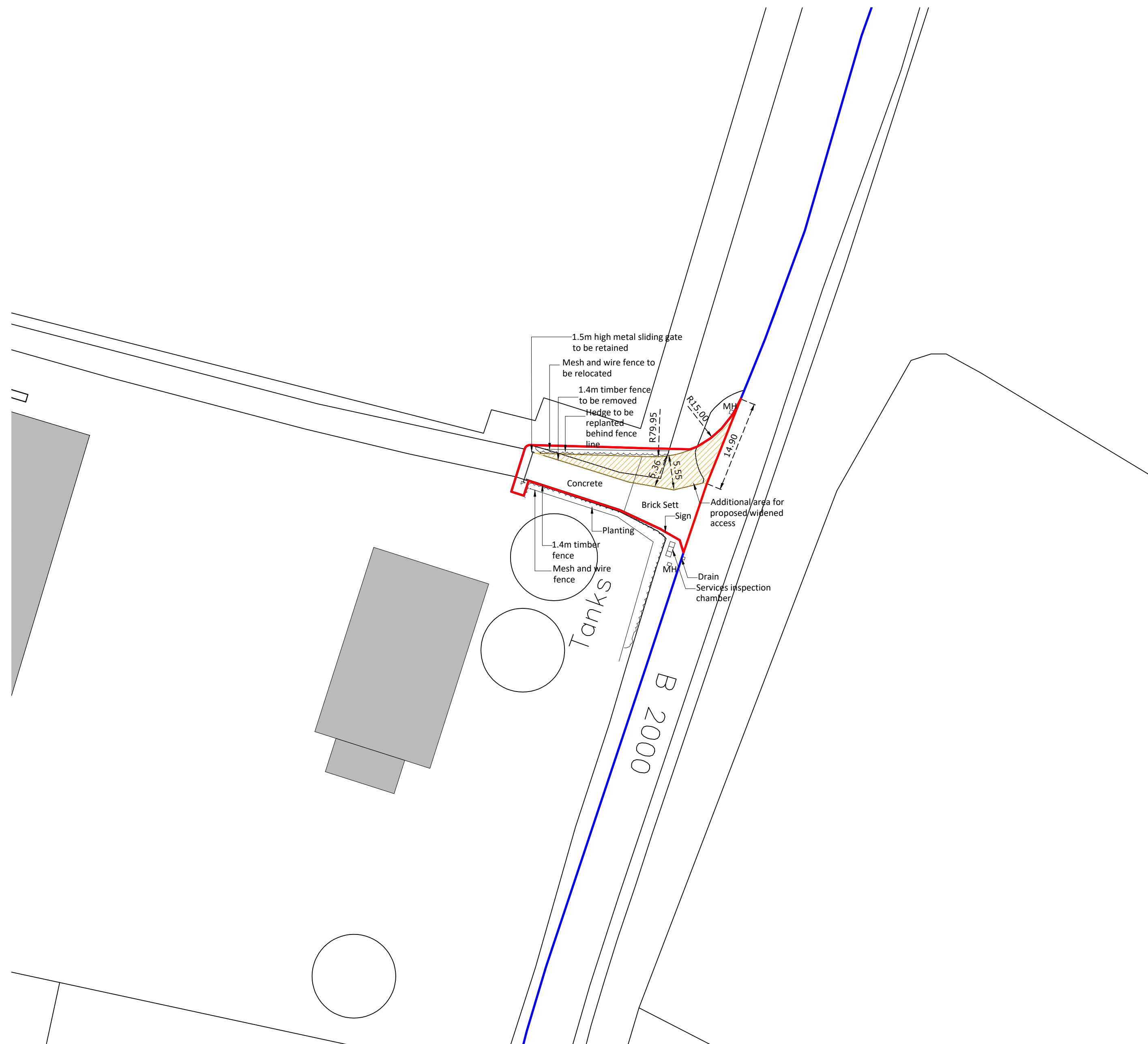
Proposed Block Plan 1:500
