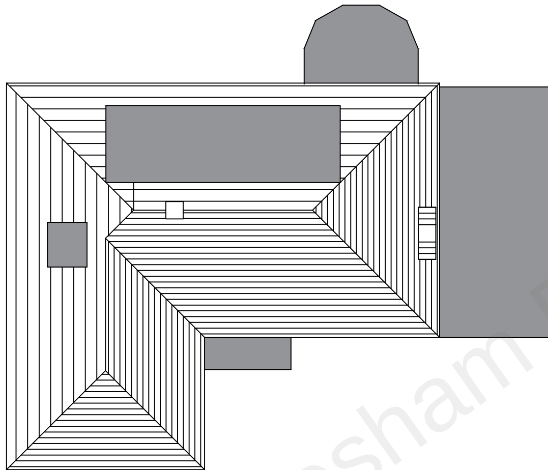
Roof Plan
