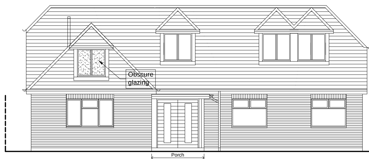
West Elevation
