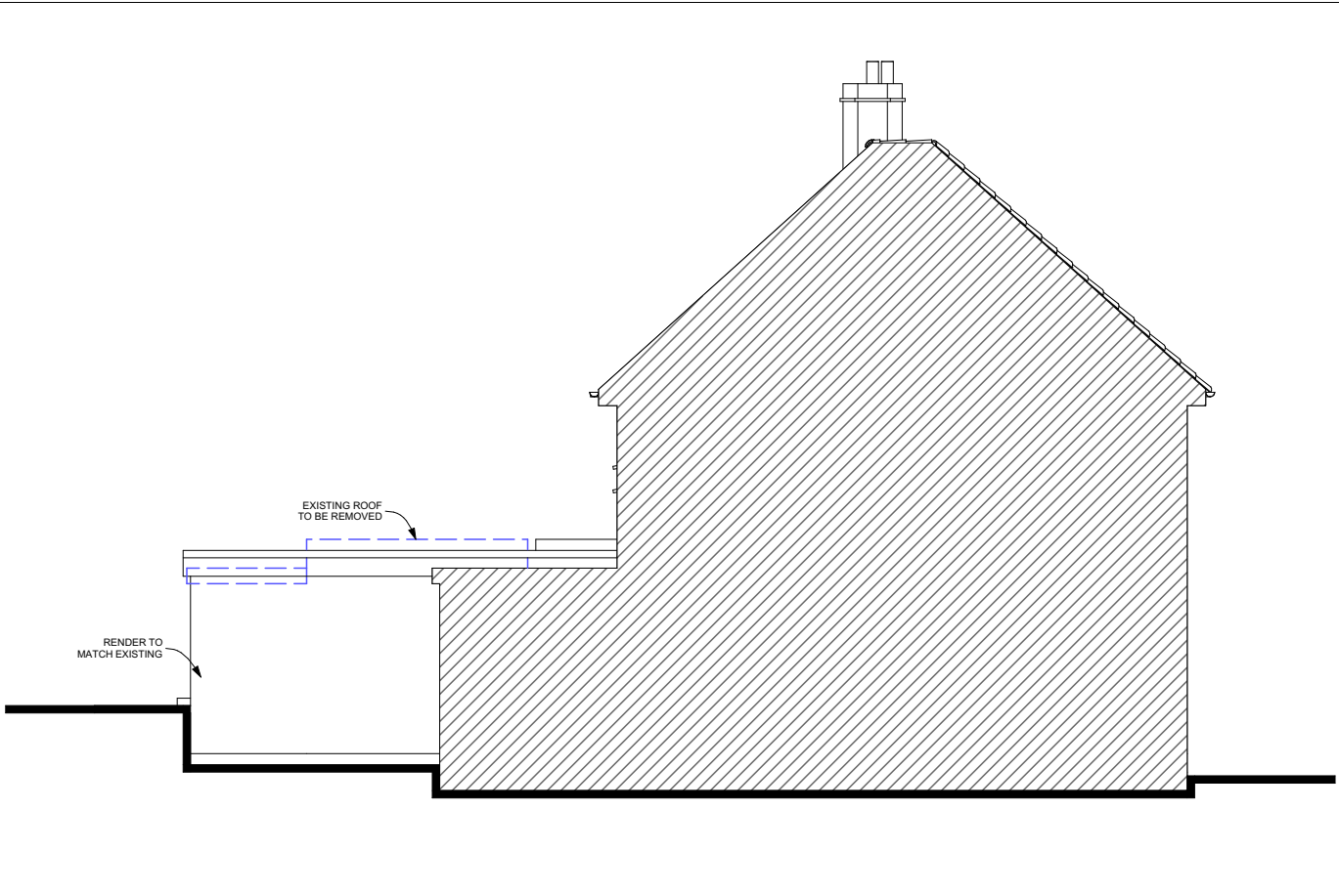
SIDE (EAST) ELEVATION PROPOSED
