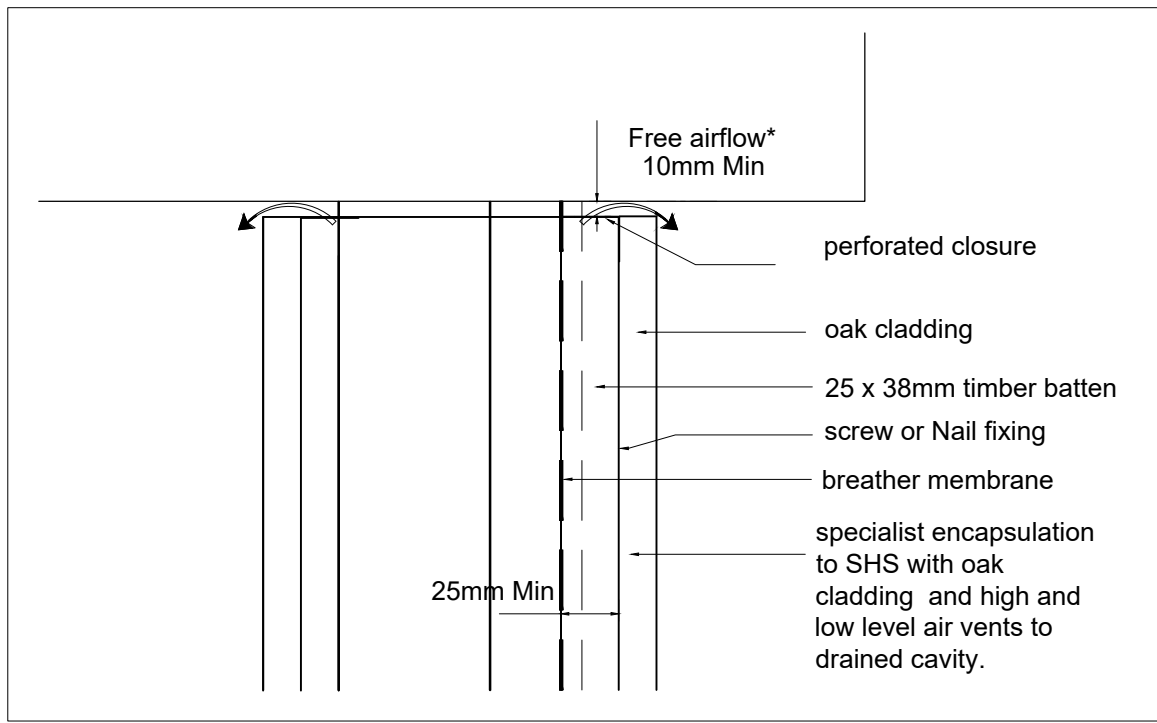
DETAIL 4 cavity vent to head and base of oak post
