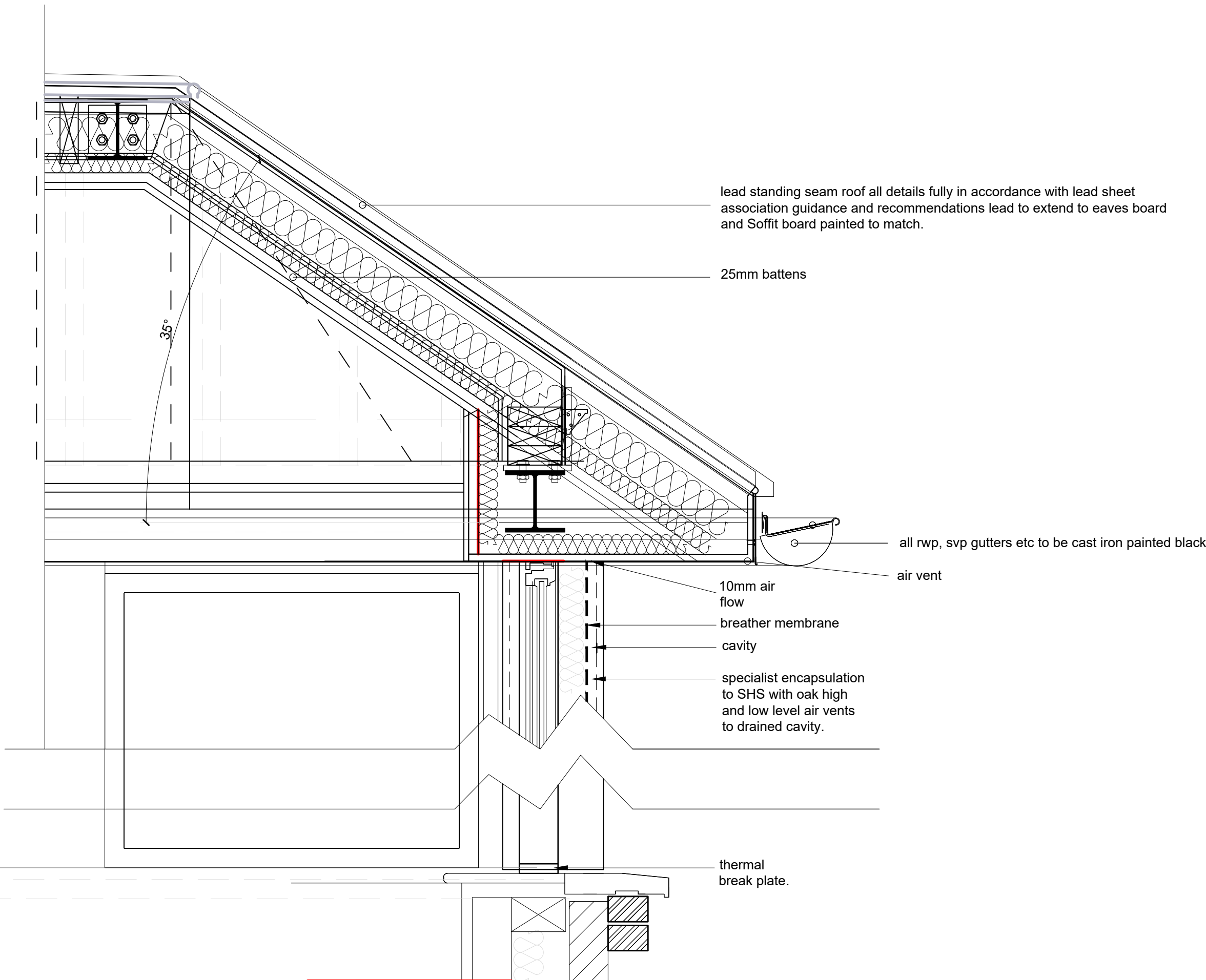
SECTION THROUGH ROOF INTERFACE
