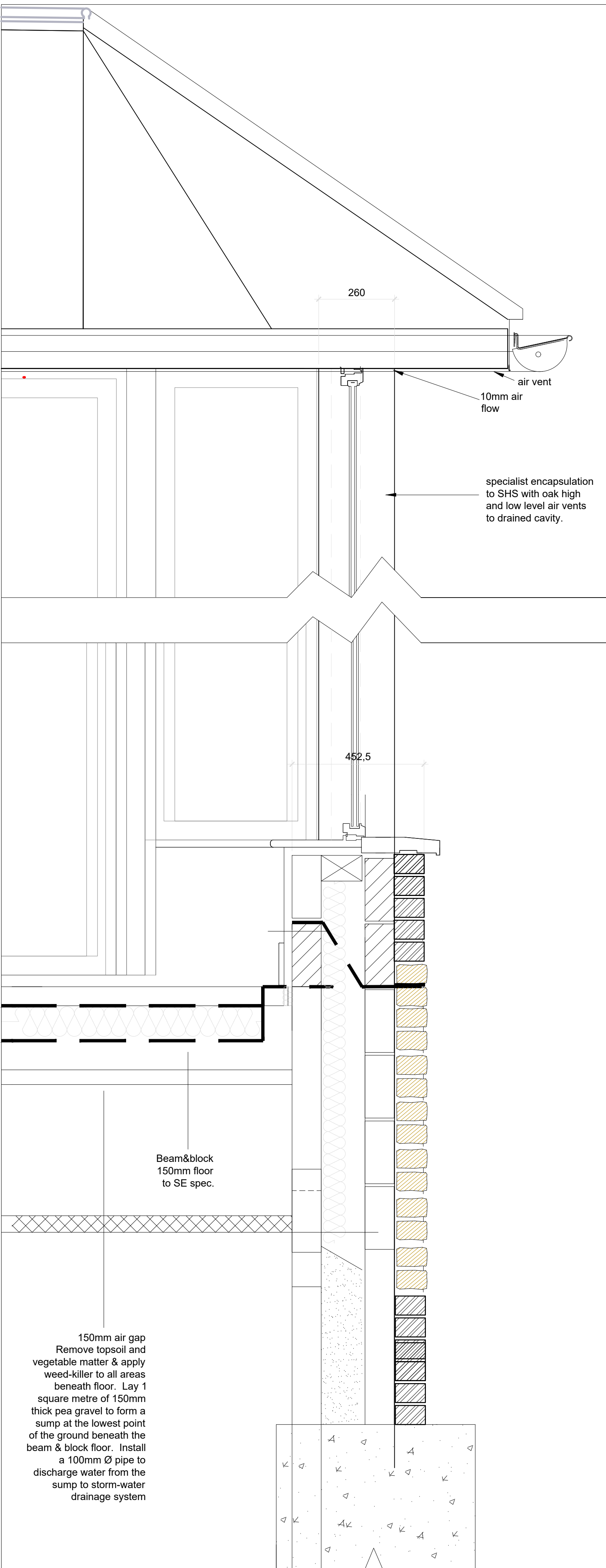
PART SECTION D - D
