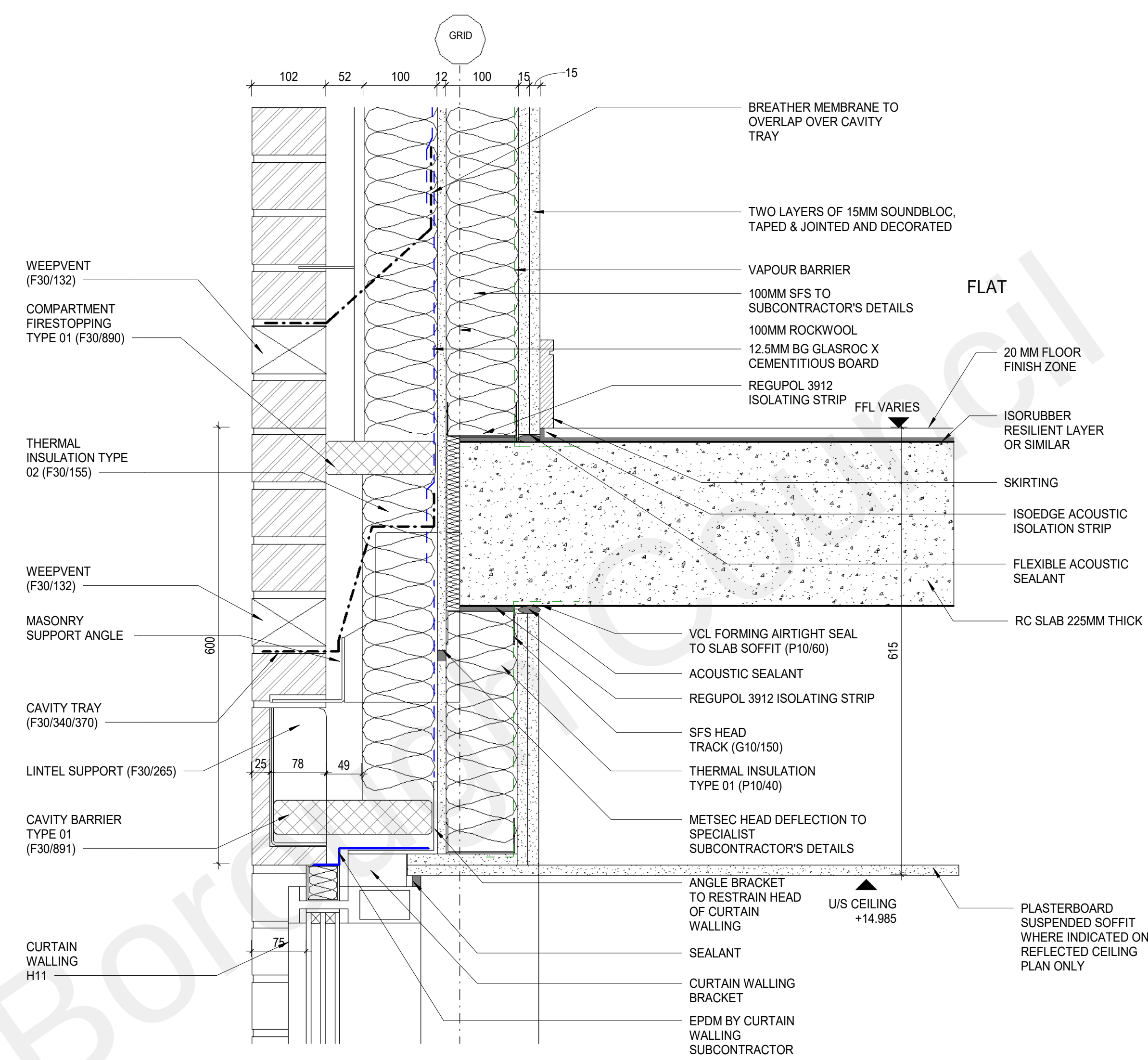
2 CURTAIN WALLING HEAD DETAIL IN BRICKWORK DETAIL EXTENDED SPAN
