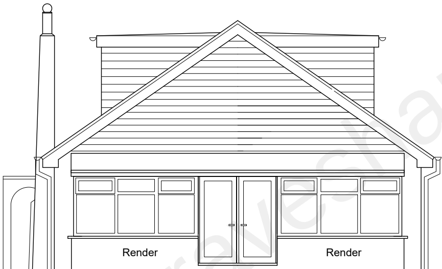
Existing Rear (North) Elevation
