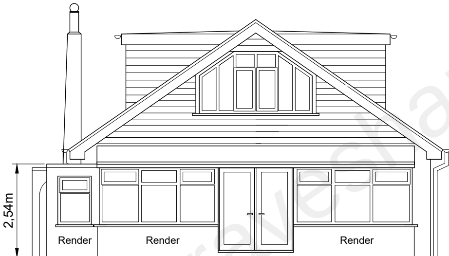
Proposed Rear (North) Elevation
