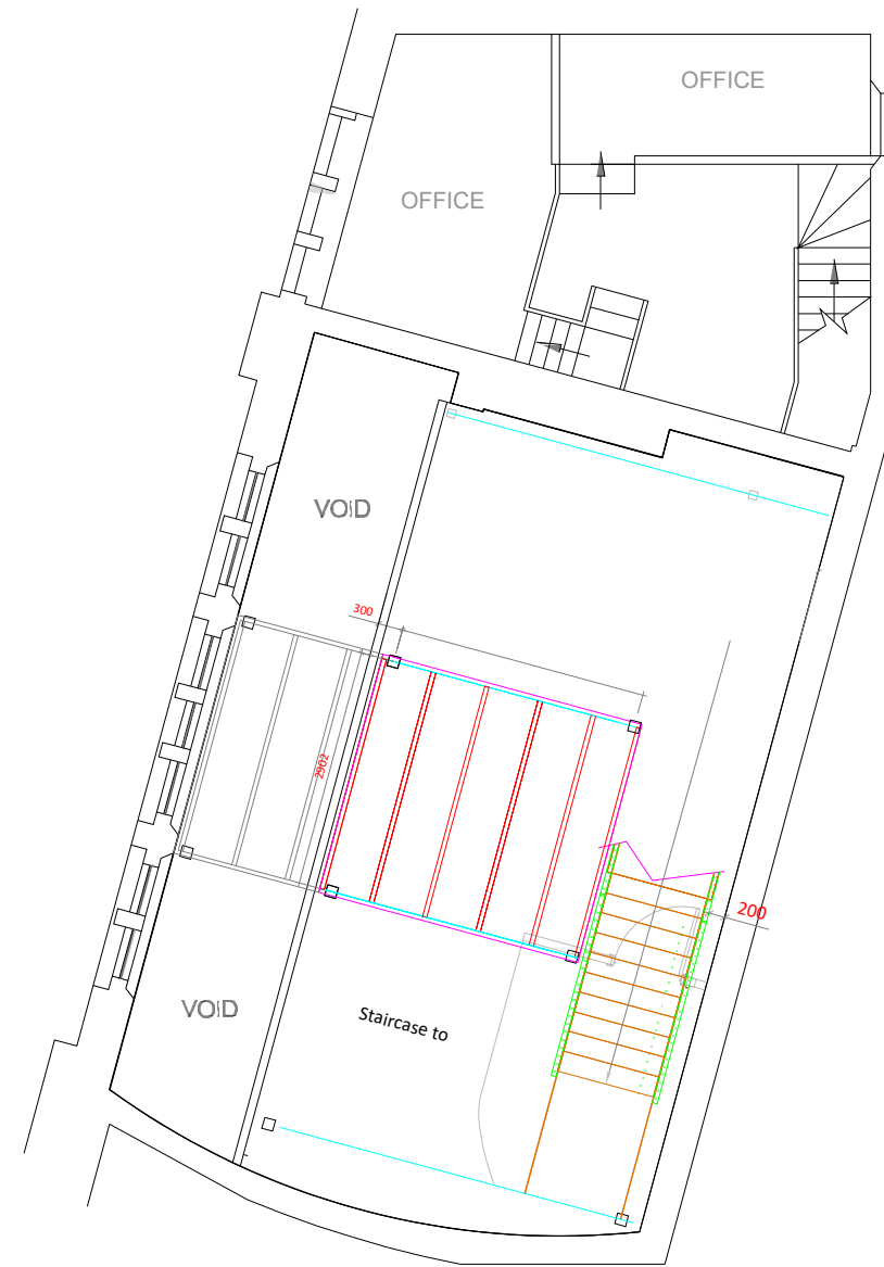
Mezzanine Floor Plan As Proposed
