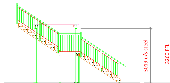
Staircase Section View
