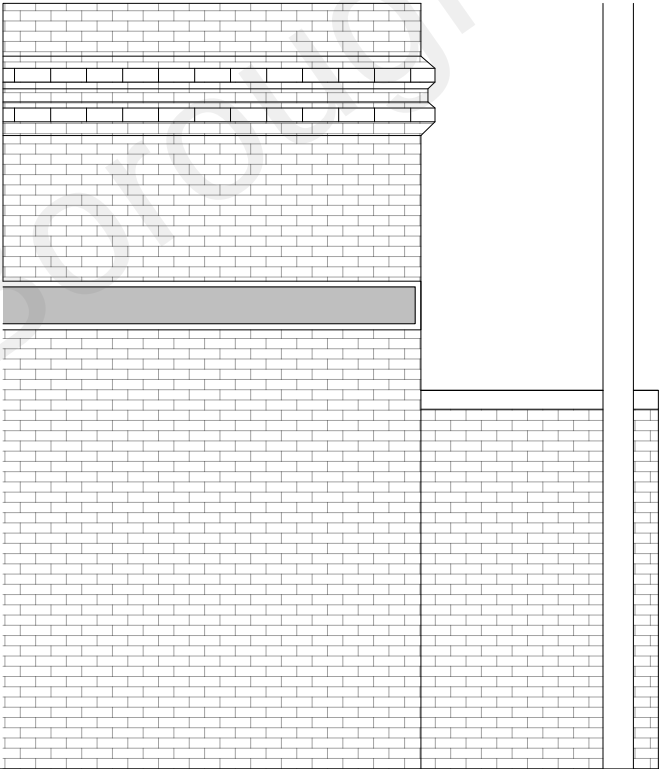
EXISTING ELEVATION B SCALE 1:50
