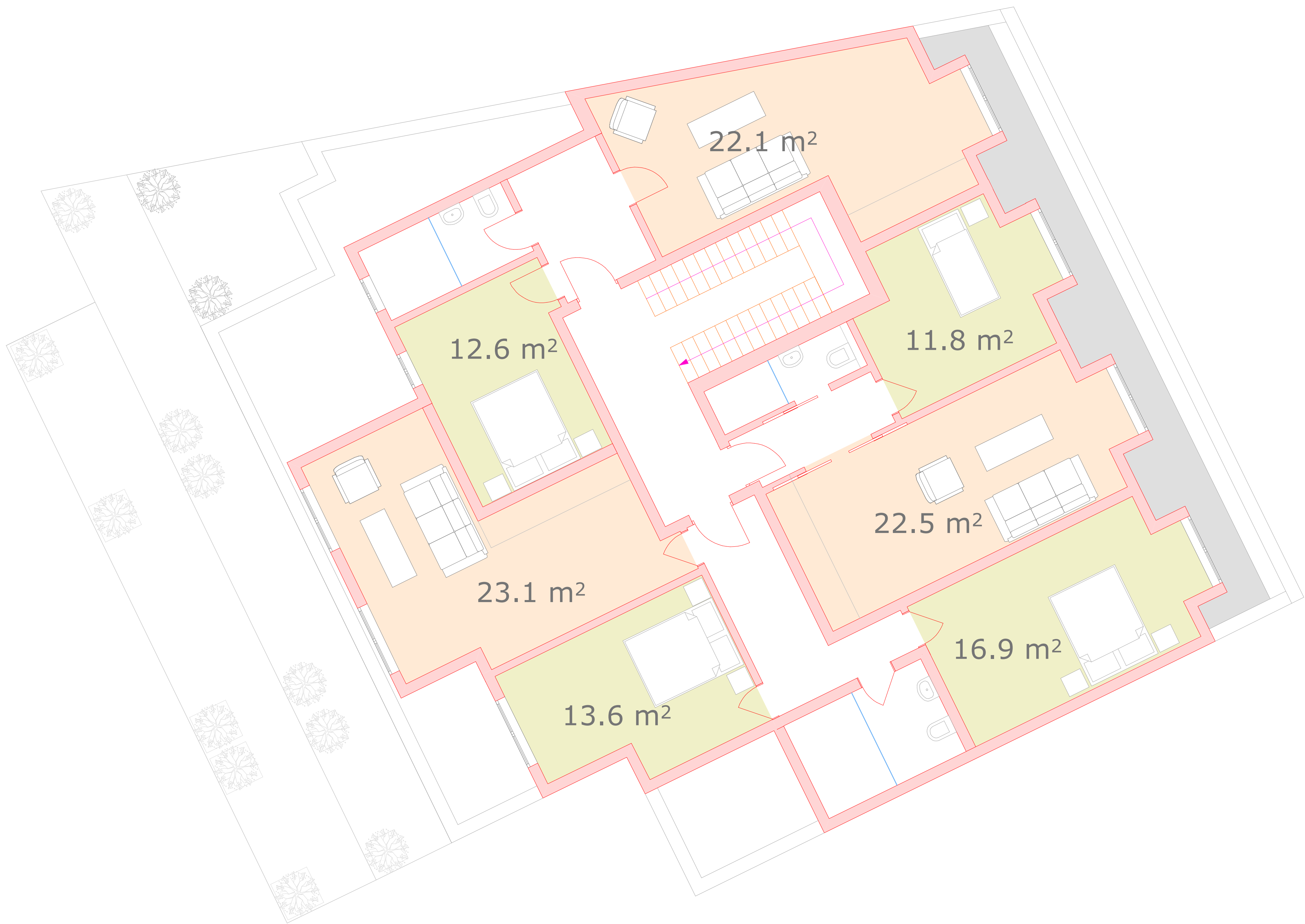
ROOF PLAN AS PROPOSED @ 1 : 50
