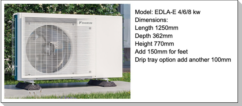
~ ASHP DETAILS ~
