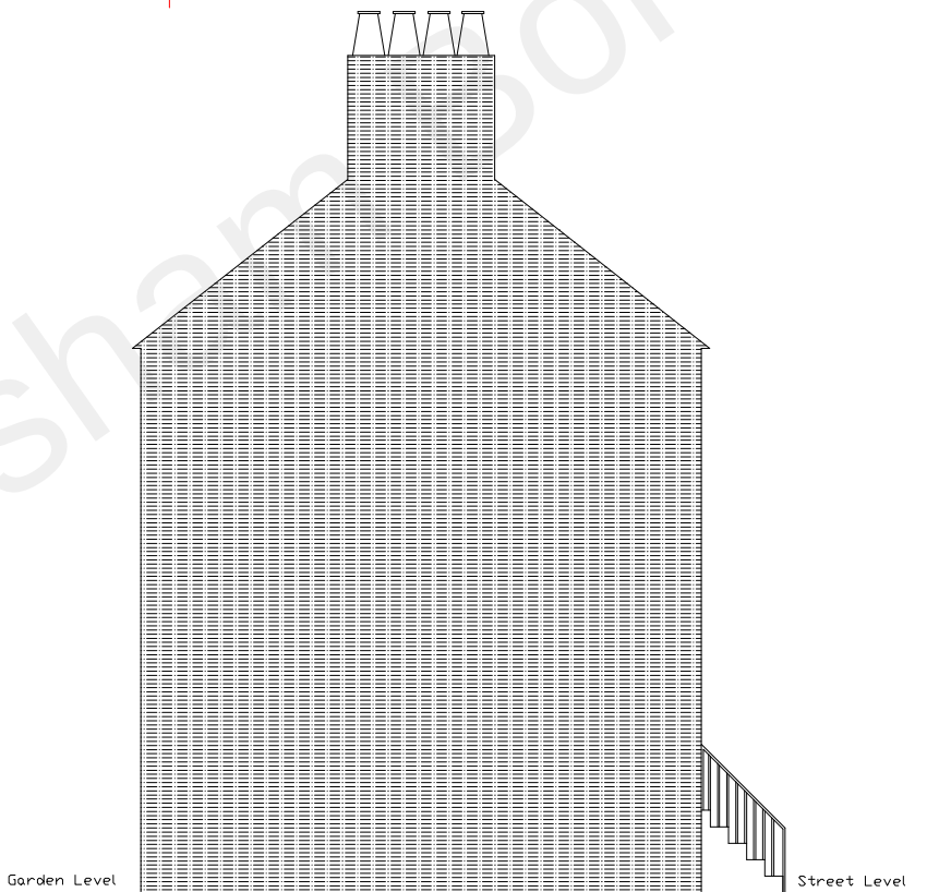
EXISTING SIDE A ELEVATION
