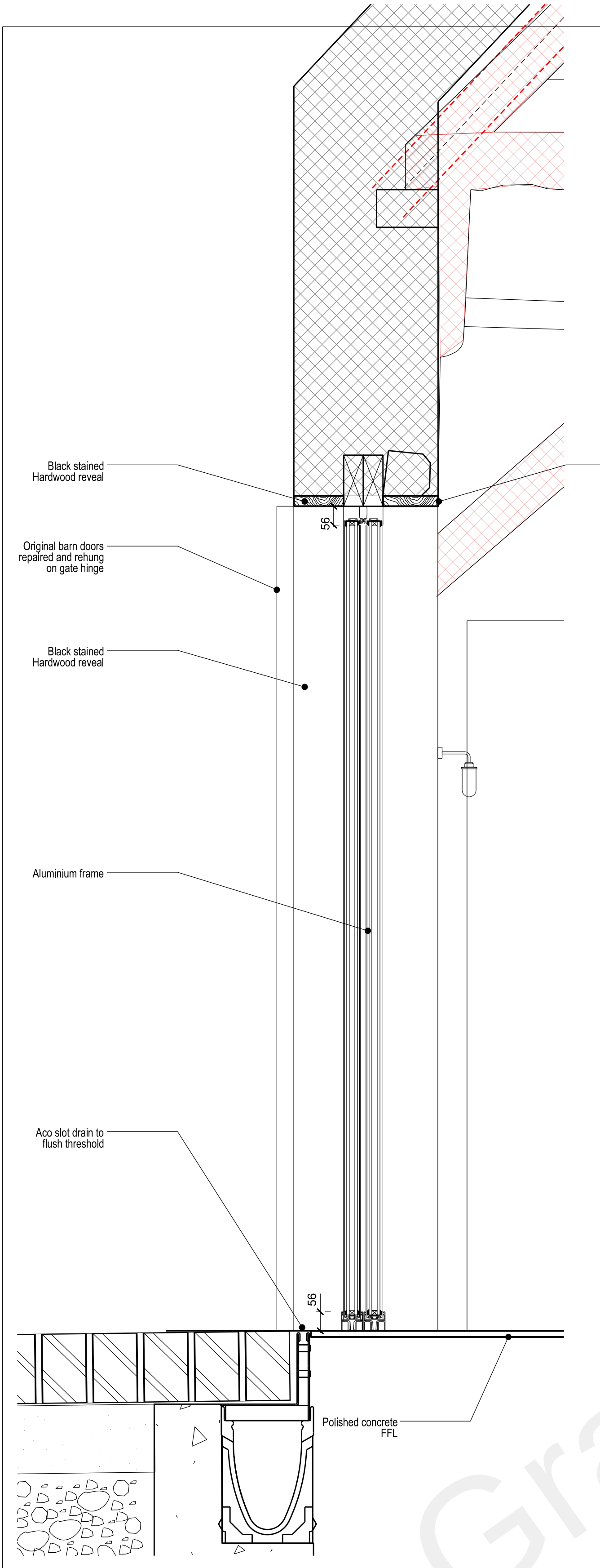
DETAIL - GF.W.01
