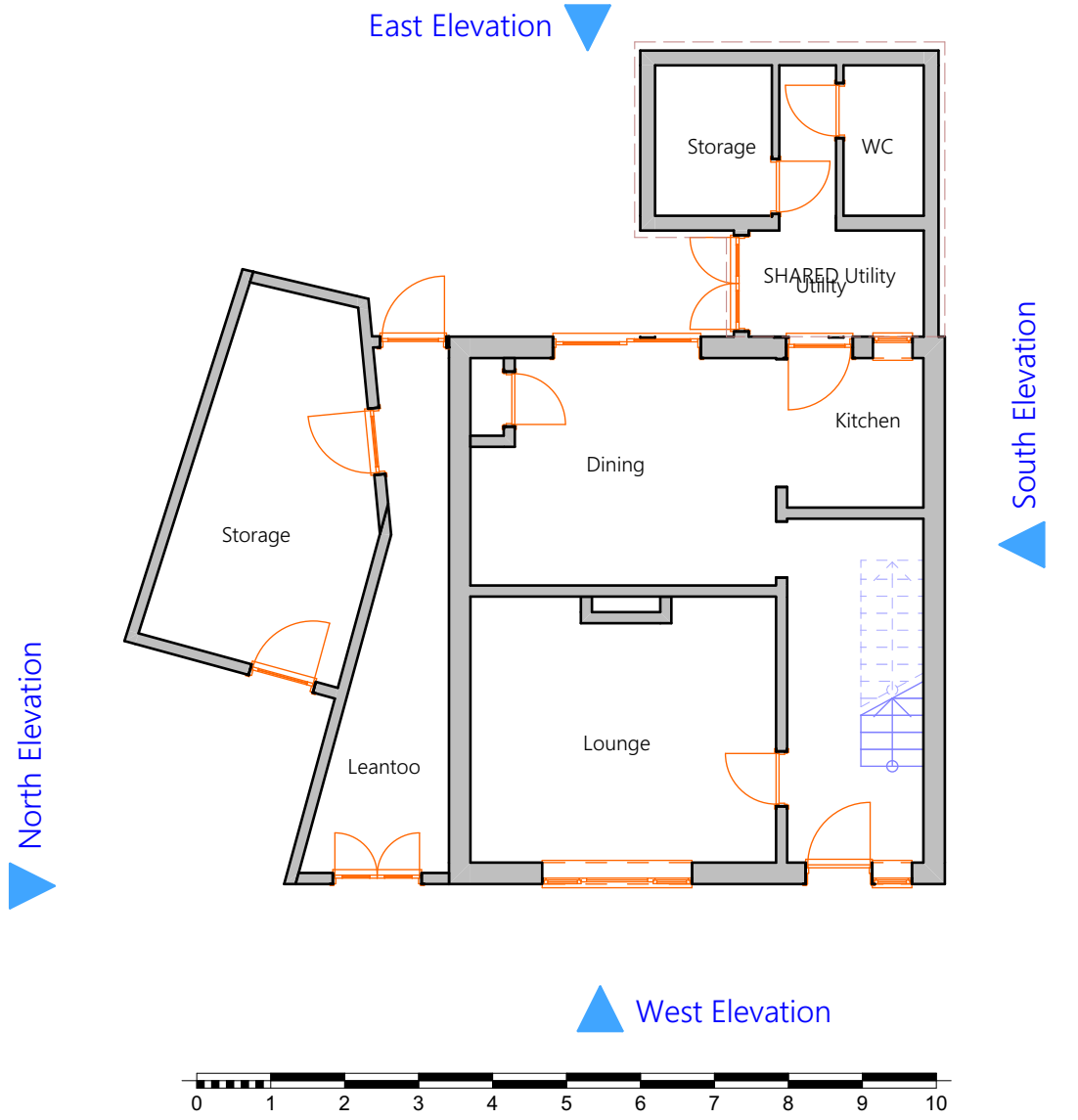
5 GF Ground Floor Existing 1:100
