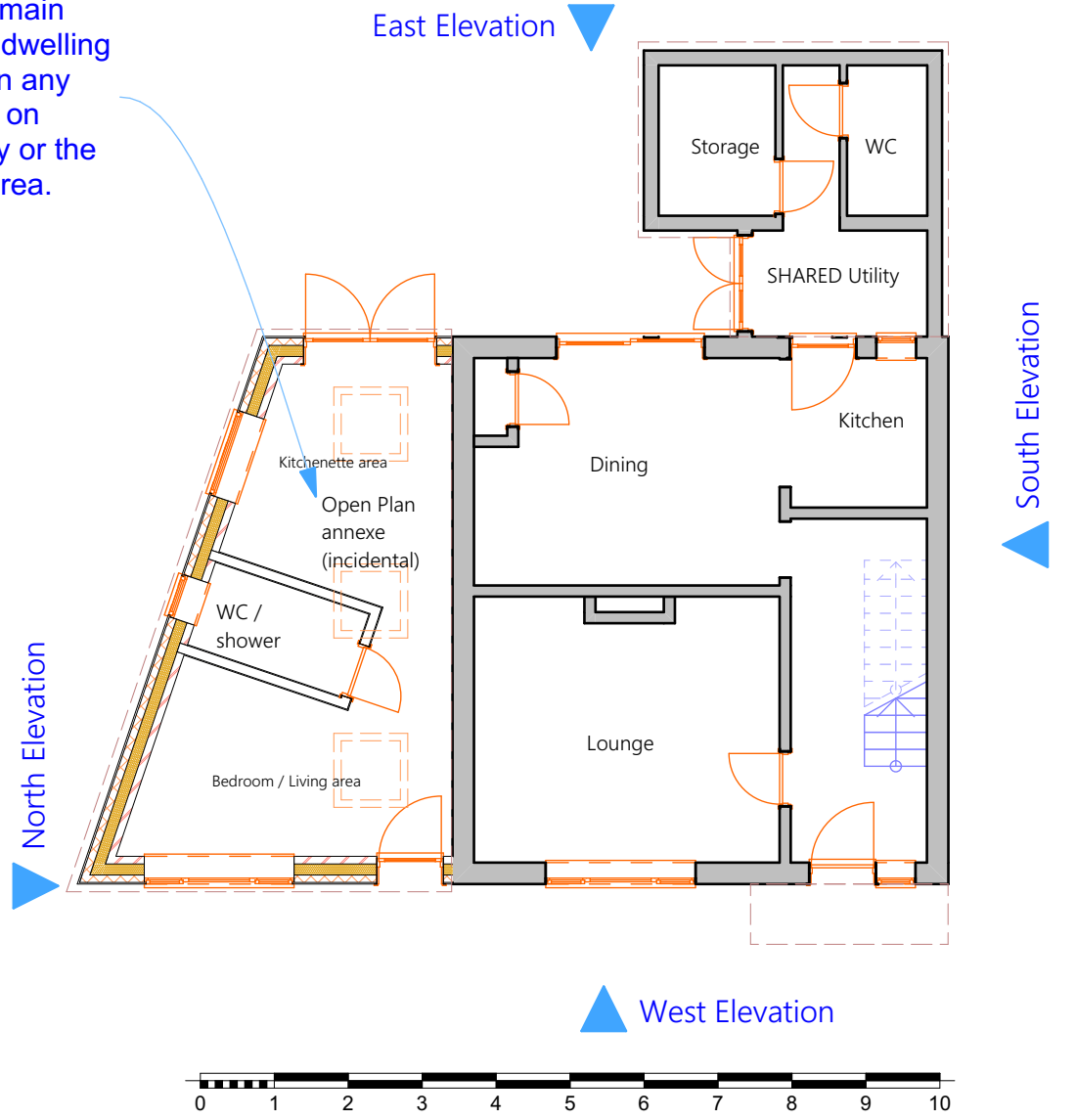
12 GF Ground Floor Proposed 1:100
