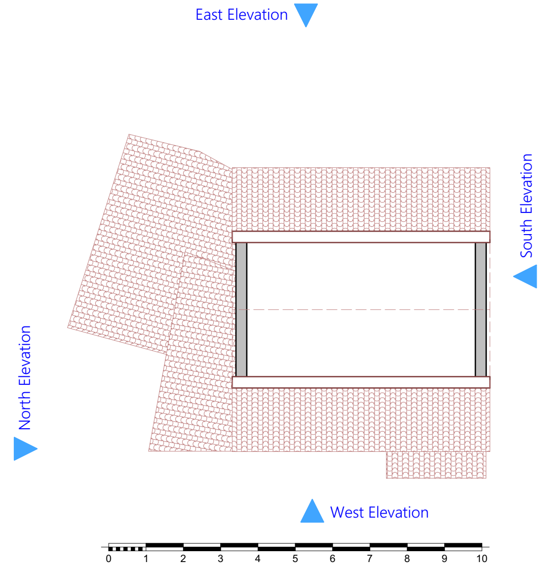
7 Roof -Existing 1:100
