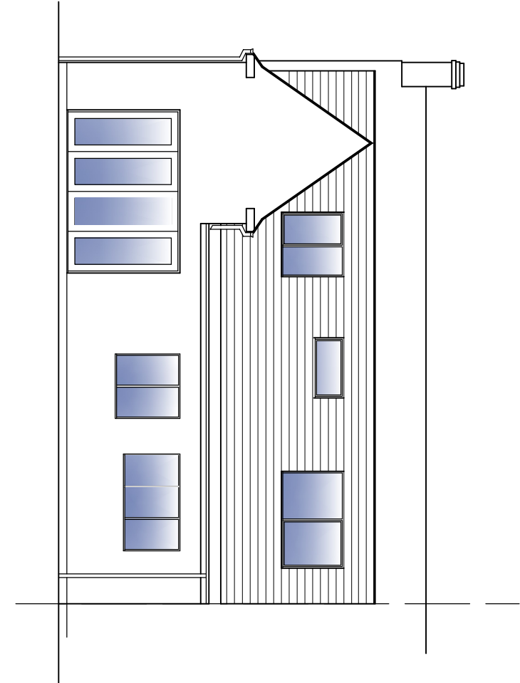
SIDE SECTIONAL ELEVATION
