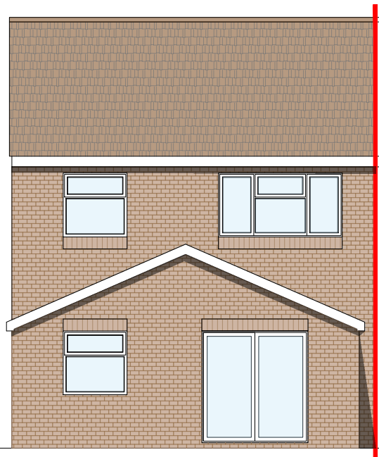
Rear Elevation
