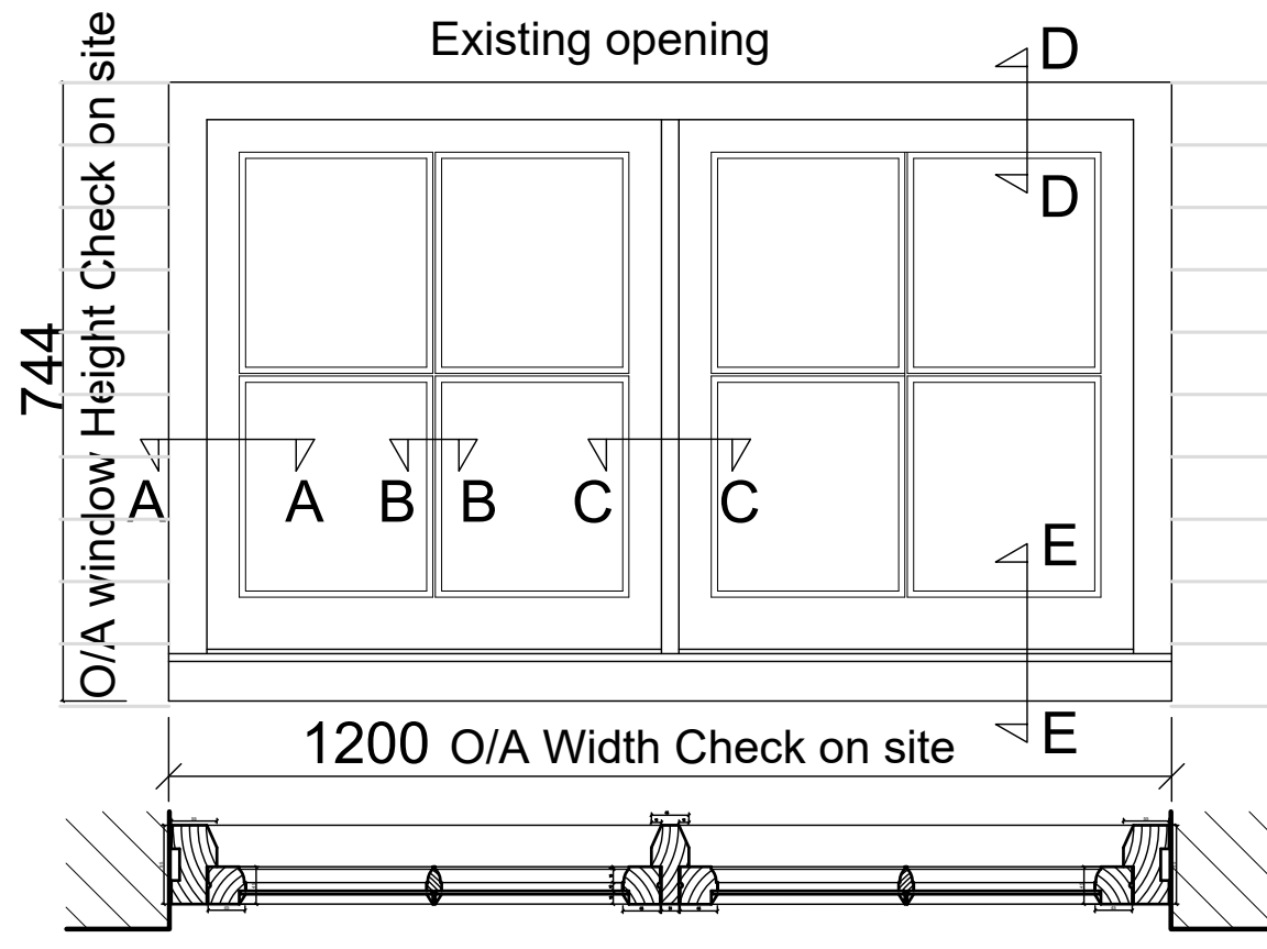
Plan (Scale 1:10)
