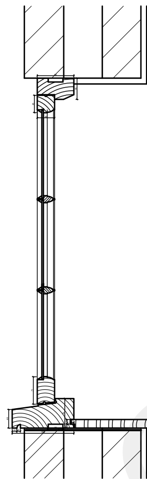
Section (Scale 1:10)
