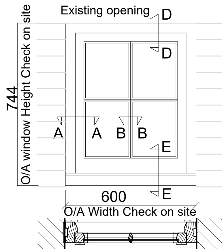
Plan (Scale 1:10)
