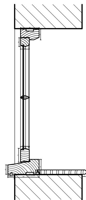
Section (Scale 1:10)
