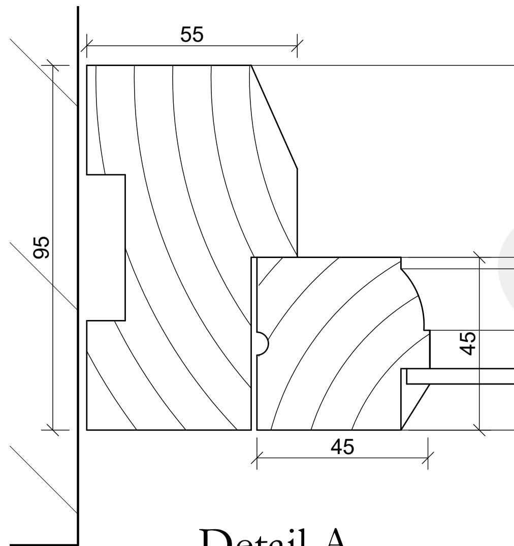
Detail A
