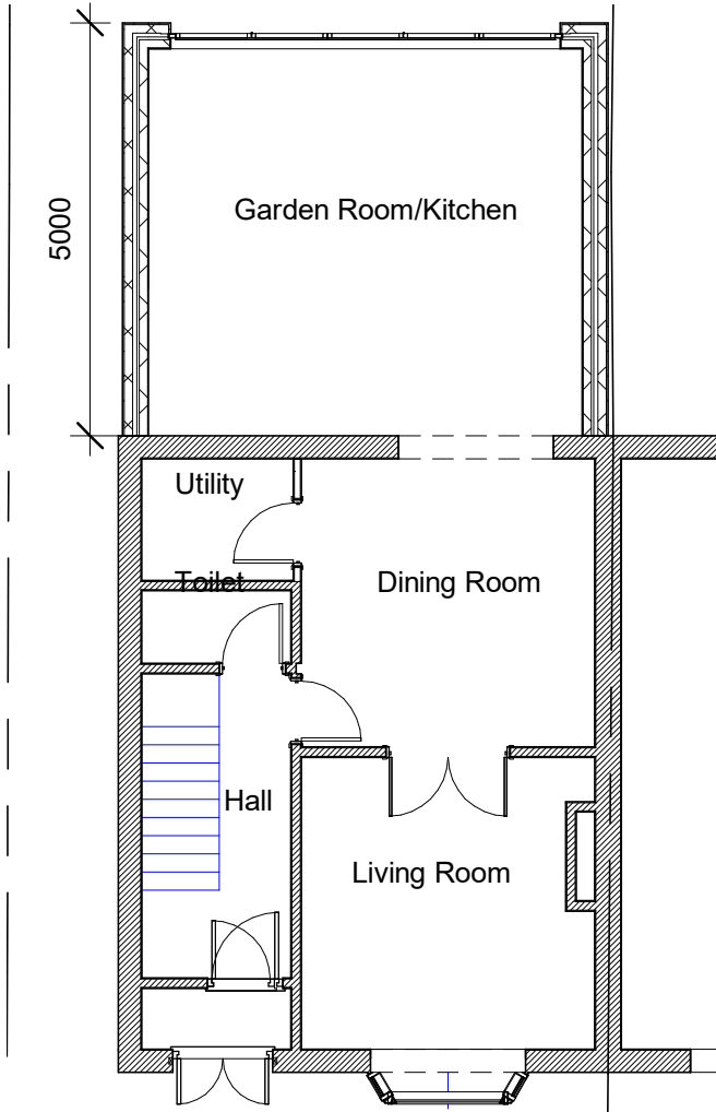
0 Pr Ground Flr 1 : 100
