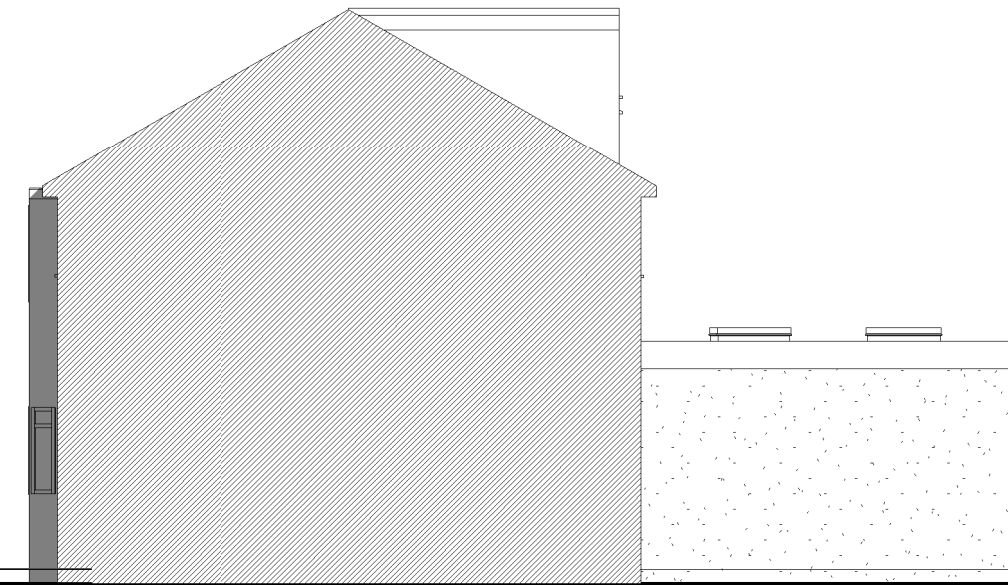
Pr Side Elevation 36 1 : 100
