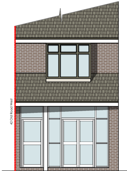
Existing Front Elevation 1:100
