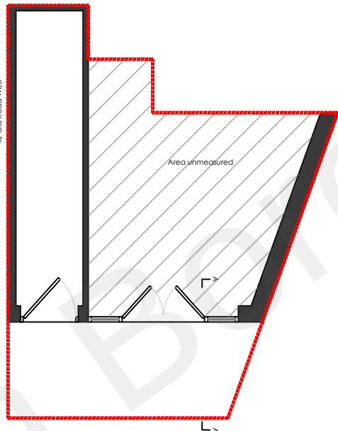
Existing Floor Plan 1:100
