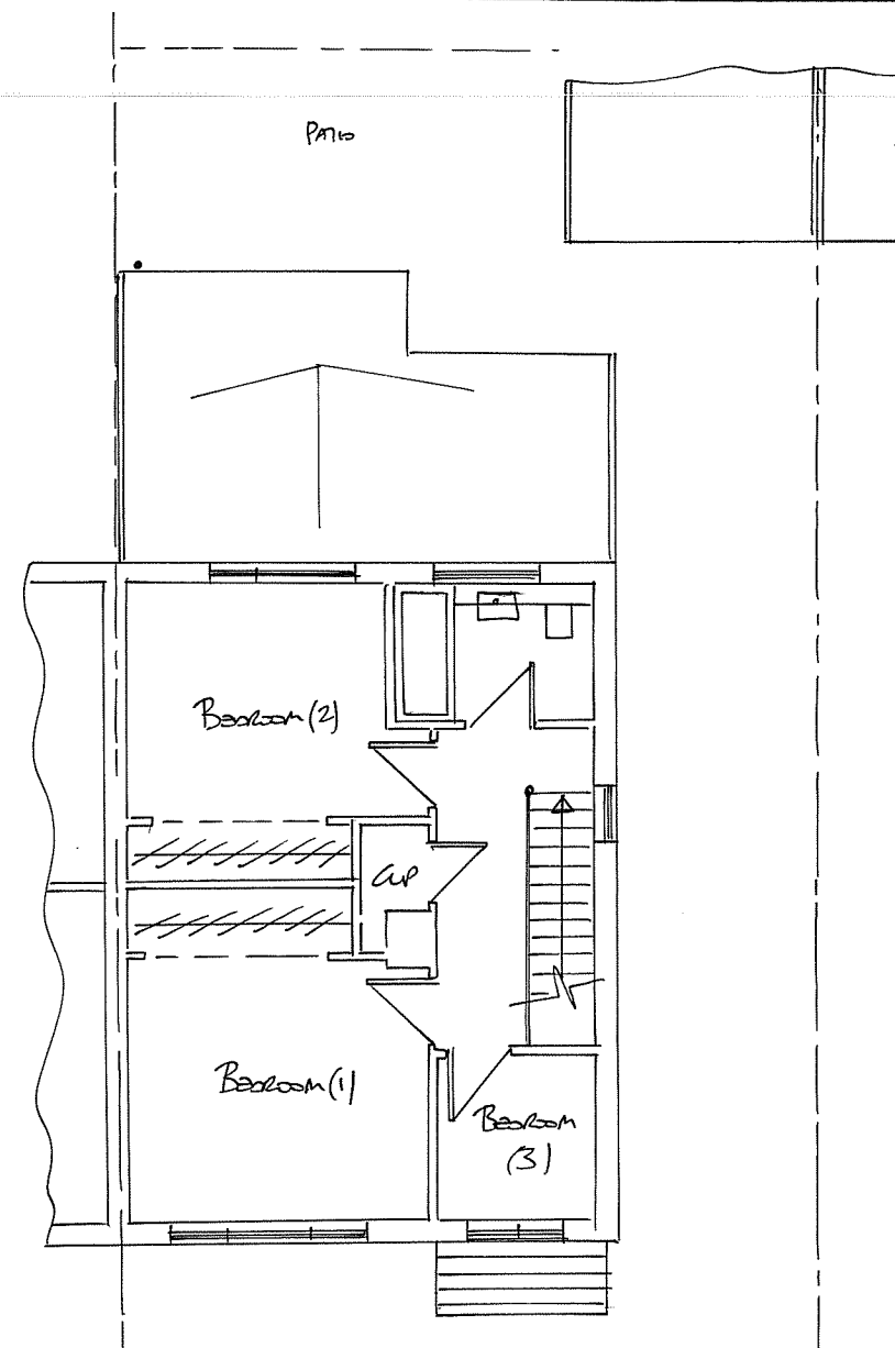
EXISTING FIRST FLR GA
