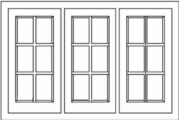
Proposed W10 Rear Elevation 1:20 @ A3
