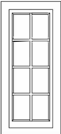
Proposed W4 Front Elevation 1:20 @ A3
