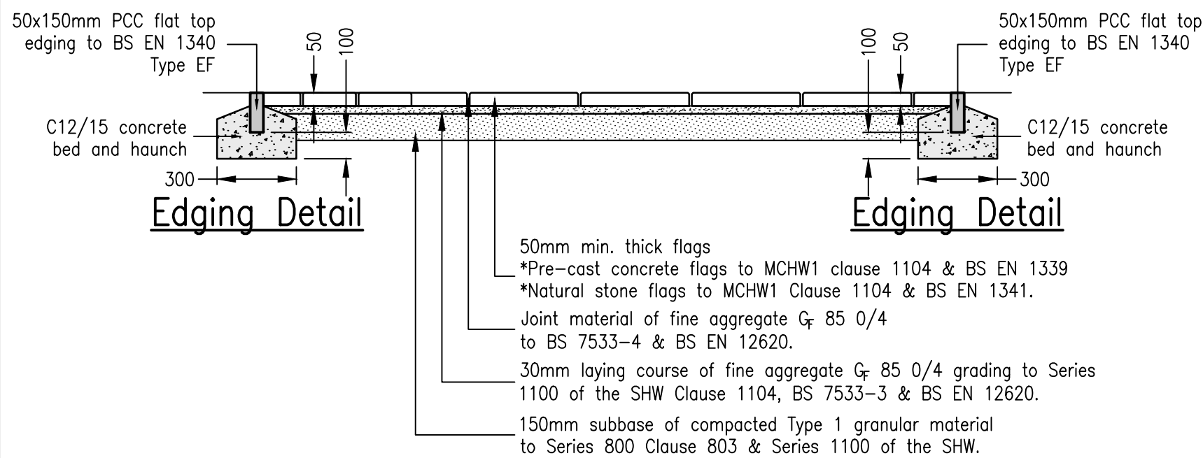
Paving Slabs – Flag Footway Construction (1:20)
