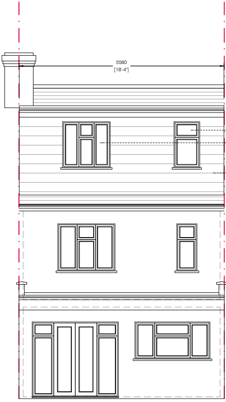
REAR ELEVATION
