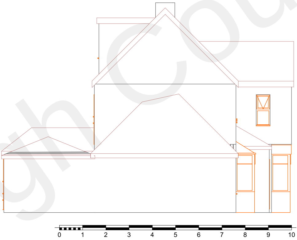
6 West Elevation Proposed 1:100
