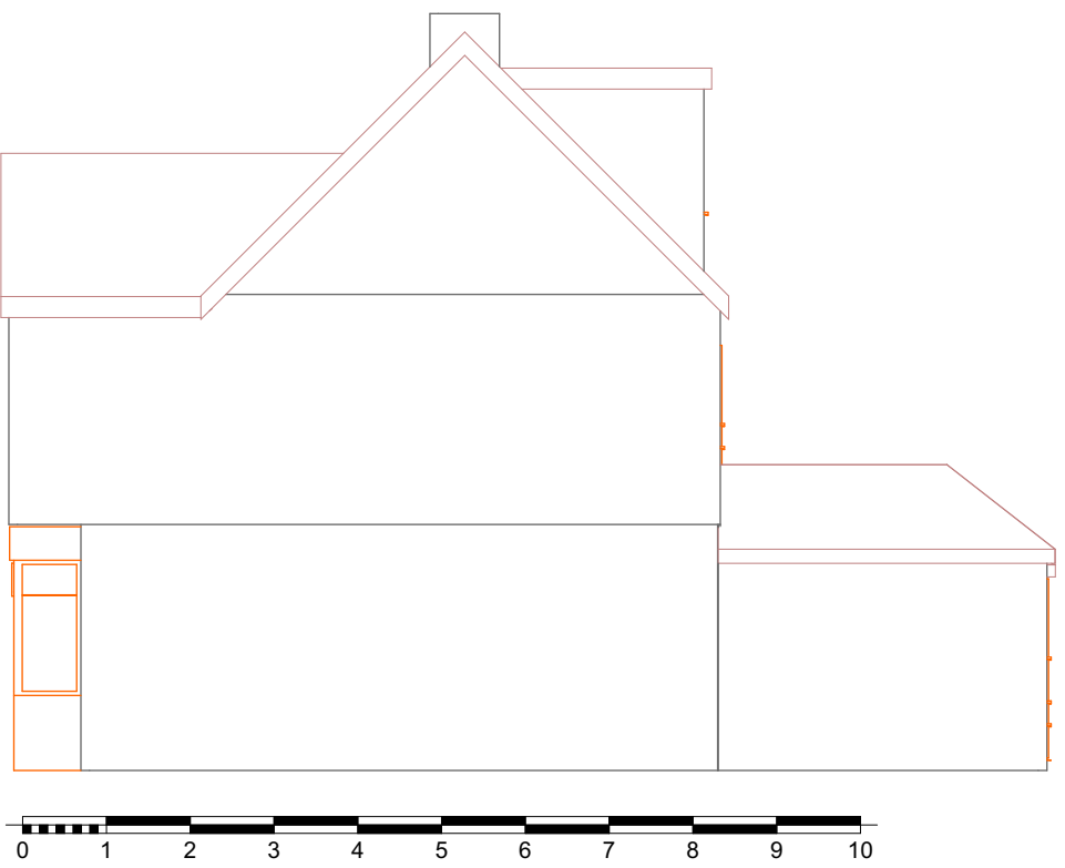
5 East Elevation Proposed 1:100
