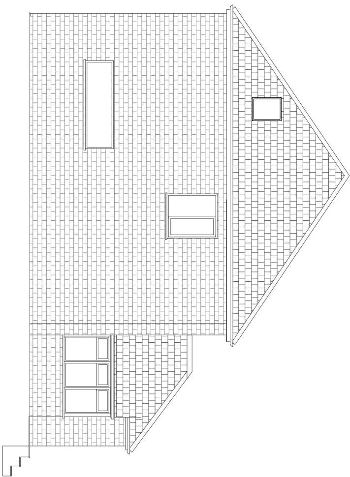
Proposed West (Side) Elevation
