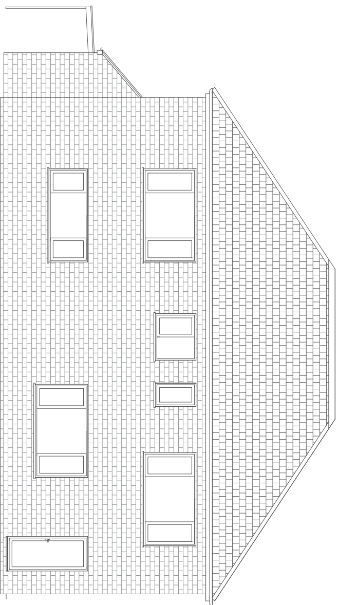
Existing South (Rear) Elevation
