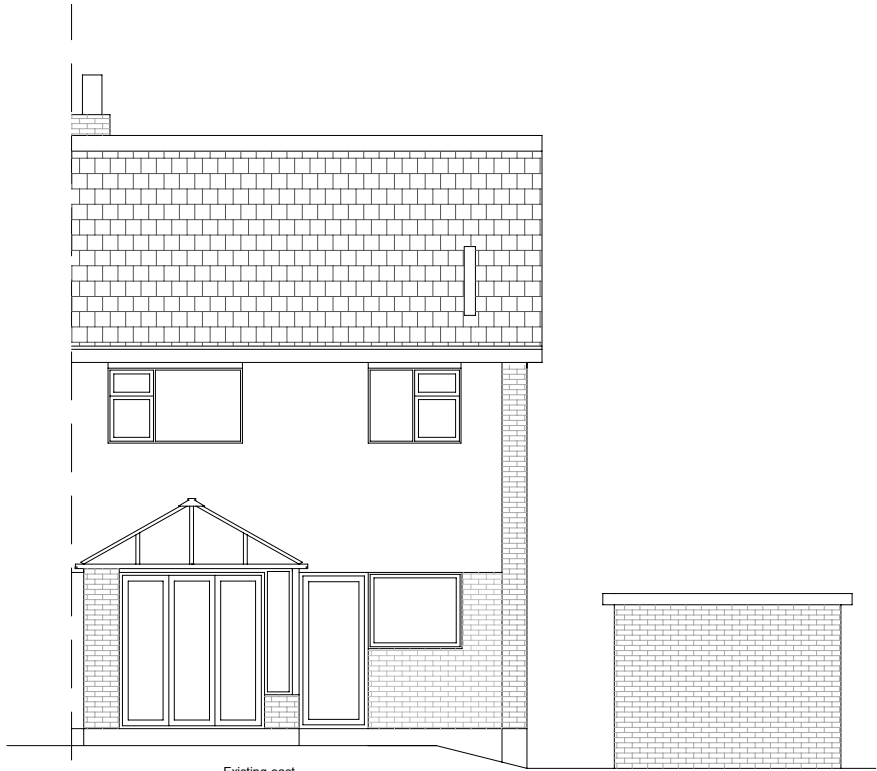
Existing east
