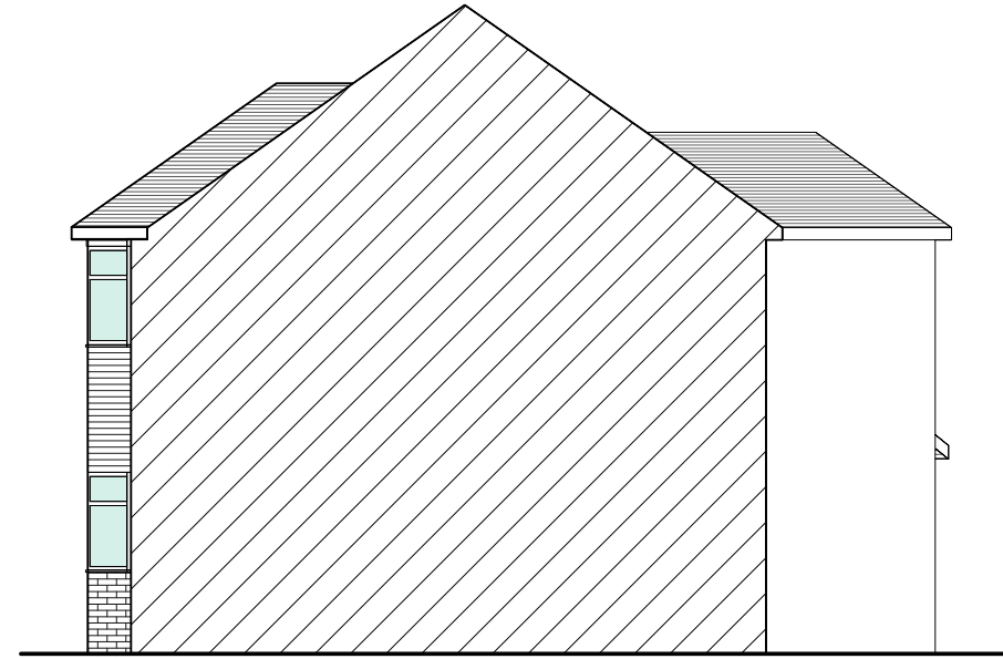
Existing LH Elevation 1 : 100
