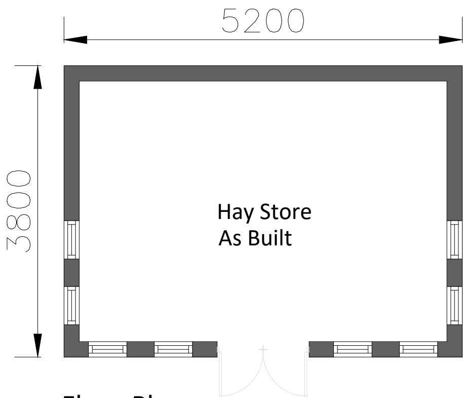
Floor Plan
