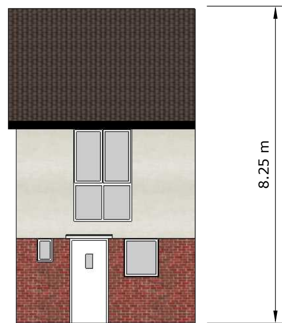
South Elevation (Principle)
