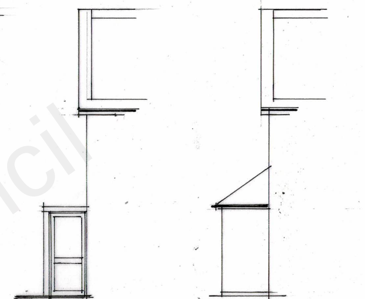
EXISTING REAR ELEV. 1:100
