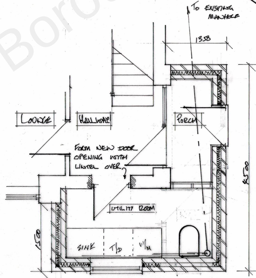
PROPOSED GROUND FLOOR PLAN 1:50
