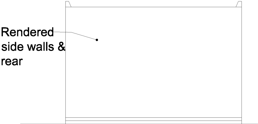
PROPOSED REAR ELEVATION B SCALE 1:50
