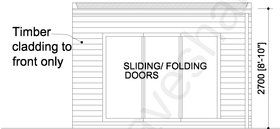
PROPOSED FRONT ELEVATION A SCALE 1:50
