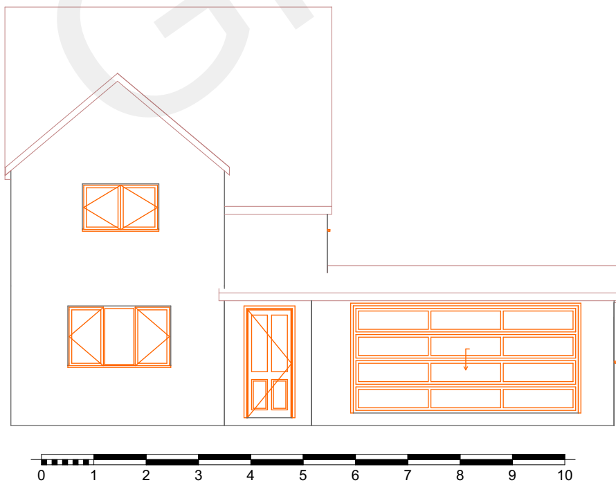
4 South Elevation Existing 1:100
