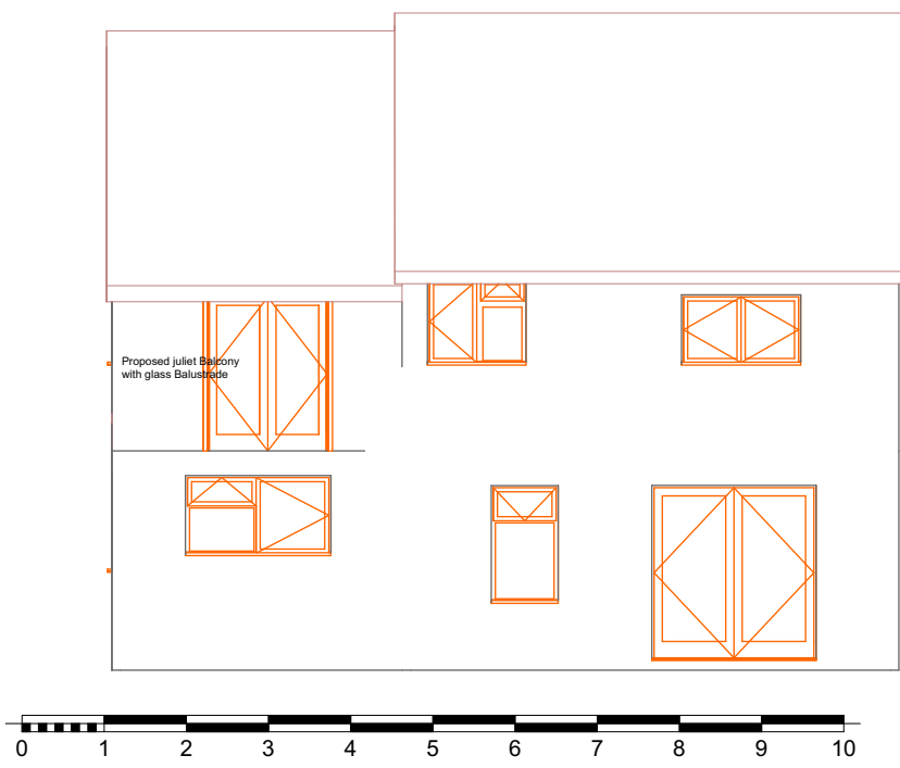
6 West Elevation Proposed 1:100
